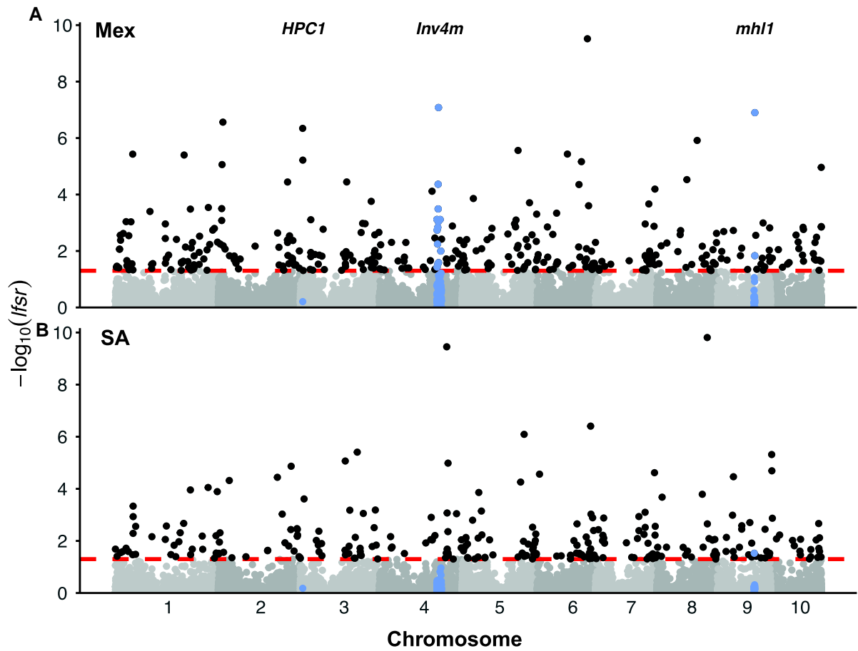
FIG. 5. Manhattan plots showing the local false sign rate ( lfsr ) of the meta-analysis with mash for detecting differential ASE between highland and lowland landraces in the (A) Mexican and (B) South American F 1 populations, expressed as -\log_{10}(lfsr) . The lfsr is analogous to a FDR but more stringent (Stephens 2017). Each dot represents a gene. The dashed line in each plot indicates the significant level at lfsr < 0.05 . Blue dots under each locus name highlight genes within the three prior-identified loci: HPC1, Inv4m and mhl1 . Mex, Mexican F 1 population; SA, South American F 1 population.
