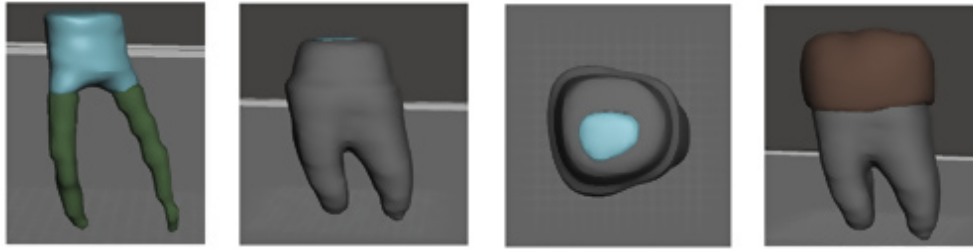
Figure 4. STL files: Core (blue), gutta percha (green), tooth structure (gray) and crown (brown).
