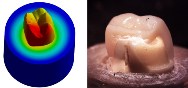
Figure 12. Correlation between total deformation (left) and fracture behavior (right) of Group I.
