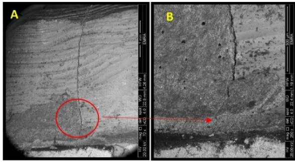
Figure 7. Mode of Failure III: SEM image revealed the crack extension through the finish line (A: 70X, B: 250X).
