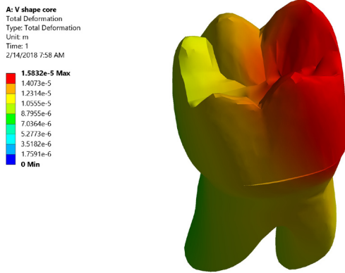
Figure 8. Color graphics showing total deformation of Group I.
