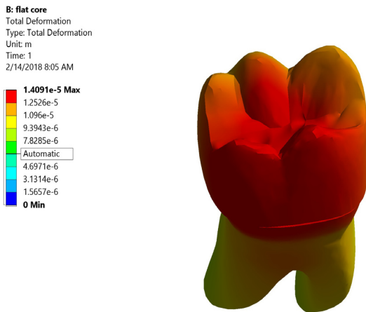
Figure 9. Color graphics showing total deformation of Group II.
