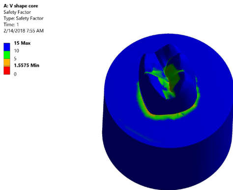
Figure 10. Color graphics showing safety factor of Group I.
