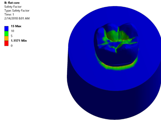
Figure 11. Color graphics showing safety factor of Group II.
