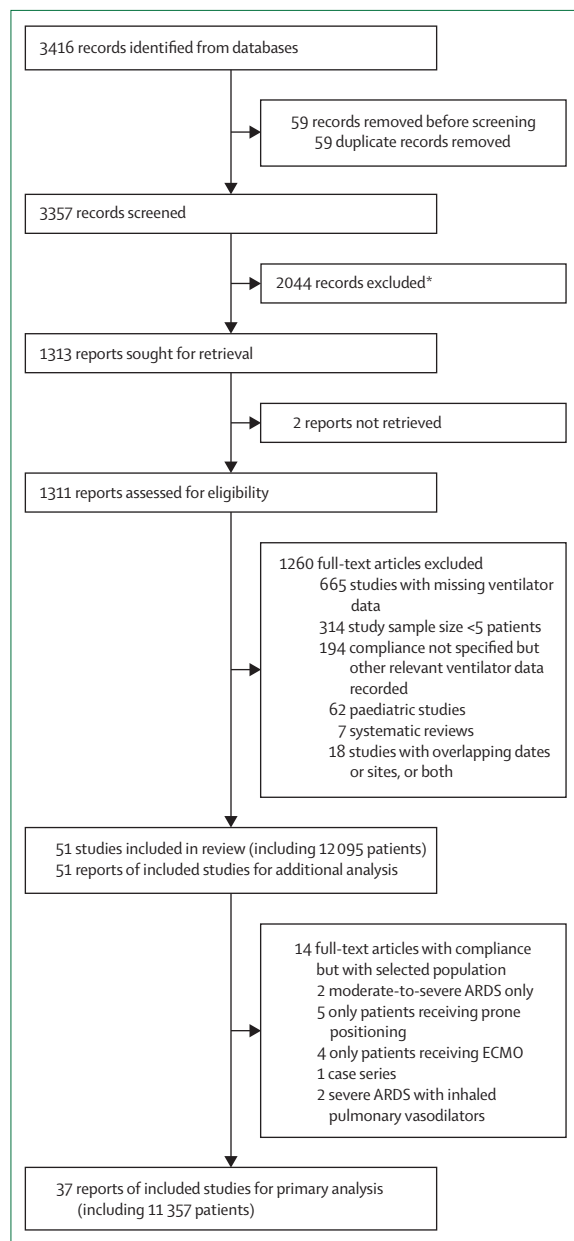
Figure 1: Study selection
