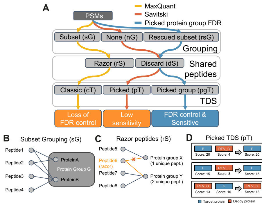
FIG. 2. Overview of protein group-level FDR estimation methods, its constituent stages, and the available options at each stage. A , a protein group-level FDR estimation method takes a list of PSMs and chooses one of the available options at each of the three stages: protein grouping, handling of shared peptides, and target-decoy strategy. B , subset grouping combines proteins into groups if the peptides of one protein (ProteinA) form a subset of the peptides of another protein (ProteinB). C , the razor peptide approach assigns a shared peptide to the protein group with the most unique identifications. D , the picked target-decoy strategy performs a target-decoy competition on protein level, retaining only the best scoring protein out of each target-decoy pair. FDR, false discovery rate; PSM, peptide-spectrum match.
