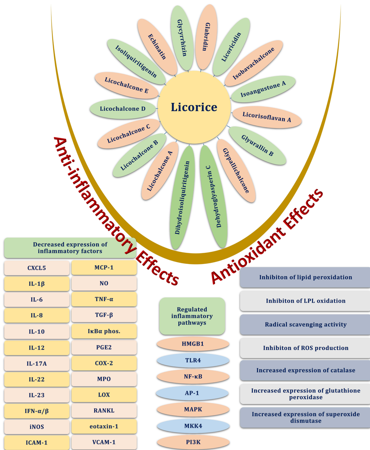
Figure 2 Anti-inflammatory and antioxidant activities of licorice and its constituents. Abbreviations: AP-1, activator protein 1; COX-2, cyclooxygenase-2; CXCL5, C-X-C motif chemokine ligand 5; HMGB1, high mobility group protein box 1; IFN, interferon; IL, interleukin; iNOS, inducible nitric oxide synthase ICAM-1, intercellular adhesion molecule 1; κBα phos, nuclear factor of kappa light polypeptide gene enhancer in B-cells inhibitor, alpha phosphate; LOX, lysyl oxidase; LPL, lipoprotein lipase; MAPK, mitogen-activated protein kinase; MCP-1, monocyte chemoattractant protein-1; MKK4, mitogen-activated protein kinase kinase 4; MPO, myeloperoxidase; NF-κB, nuclear factor kappa-light-chain-enhancer of activated B; NO, nitric oxide; PGE2, prostaglandin E2; PI3K, phosphatidylinositol 3-kinase; RANKL, receptor activator of nuclear factor kappa-B ligand; ROS, Reactive oxygen species; TGF-β, transforming growth factor-β; TLR4, Toll-like receptor 4; TNF-α, tumor necrosis factor-α; VCAM-1, vascular cell adhesion molecule 1.
