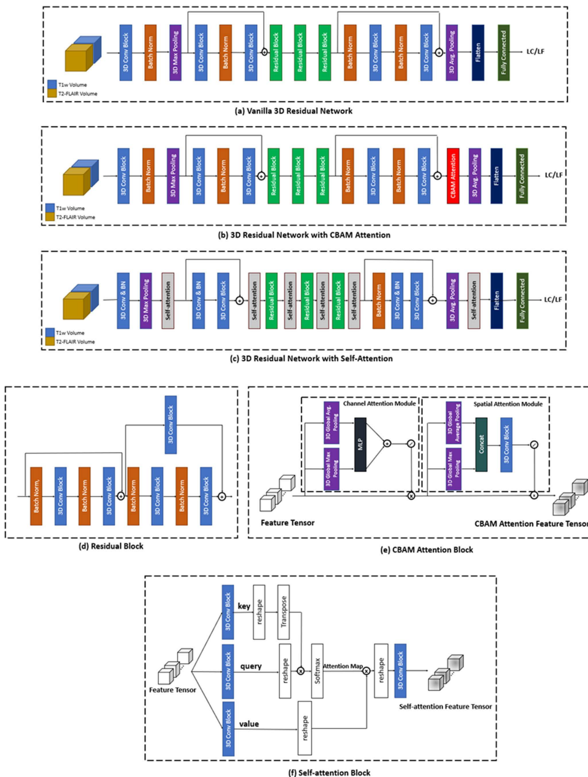
FIGURE 1. Architecture of (a) vanilla 3D residual network (baseline), (b) the 3D residual network with CBAM attention, (c) the proposed self-attention-guided 3D residual network, (d) the residual block in 3D residual network, consisting of residual connections, (e) the CBAM attention block consisting of the channel and spatial attention modules, and (f) the self-attention block consisting of the key, query, and value tensors that generates the final self-attention feature tensor.
