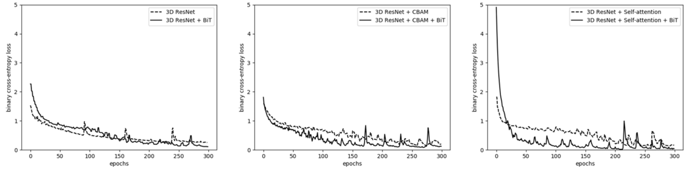
FIGURE 2. Training loss of the three models investigated in this study before and after applying BiT training scheme. Following the BiT training recipe generally led to faster convergence, smaller loss, and better performance overall.
