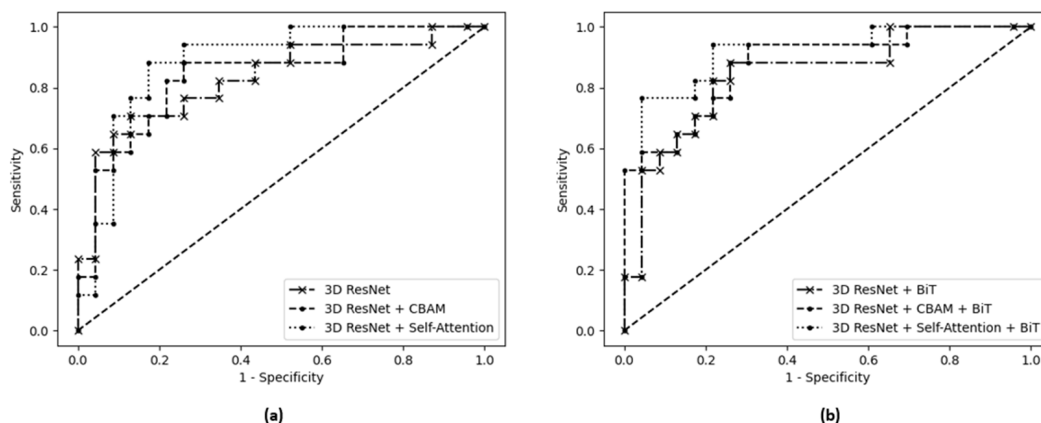
FIGURE 3. The ROC curves for (a) vanilla 3D residual network, 3D residual network + CBAM, and 3D residual network + self-attention, and (b) the same models trained with the BiT scheme.
