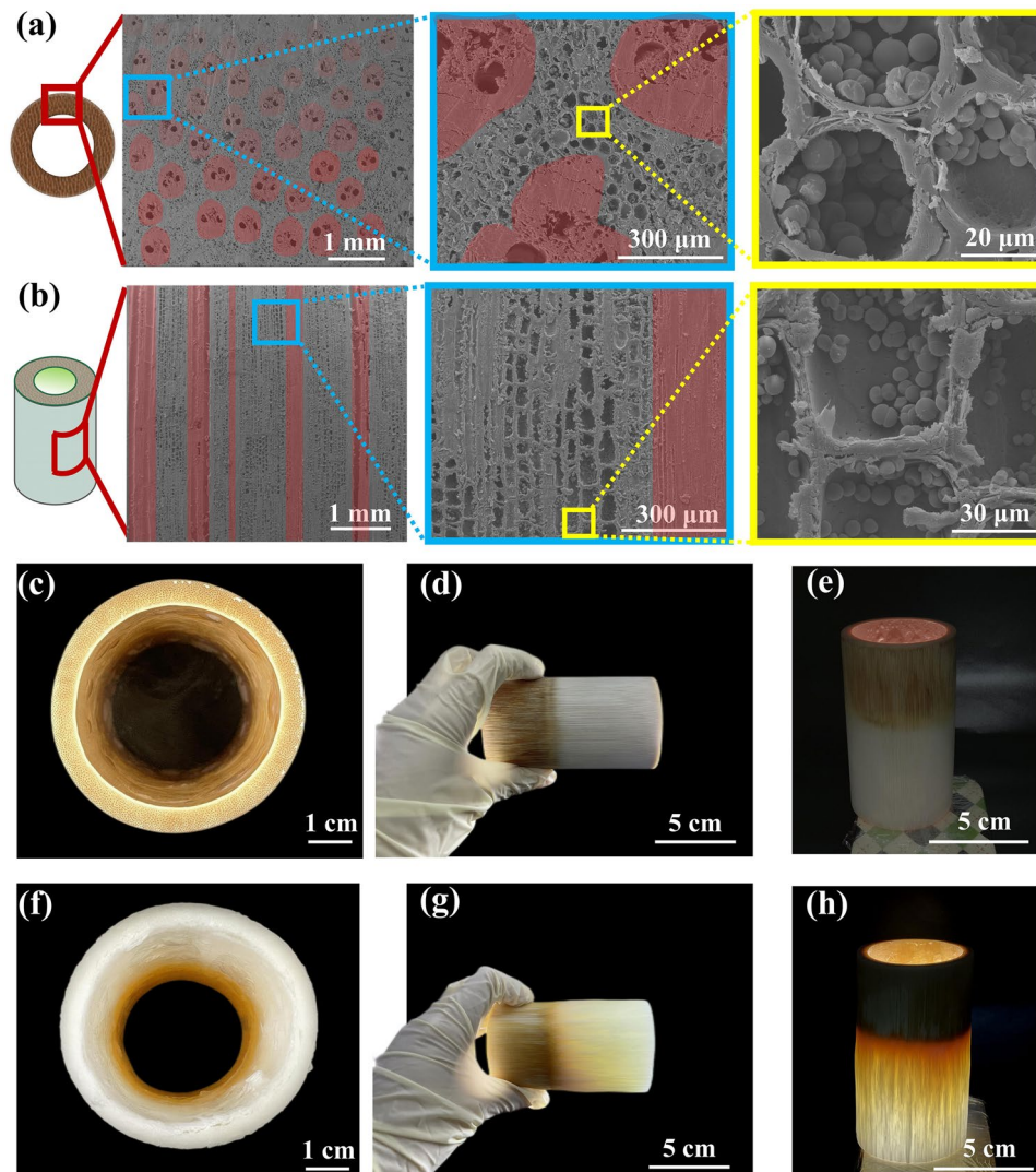
Fig. 2 a Cross-sectional SEM images of OB. b SEM images of the longitudinal section of OB. c Photograph of the cross section of S12. d Macroscopic view of S12. e Macroscopic view of S12 under the light. f Photograph of the cross section of H12. g Photograph of H12. h Photograph of H12 under the light
