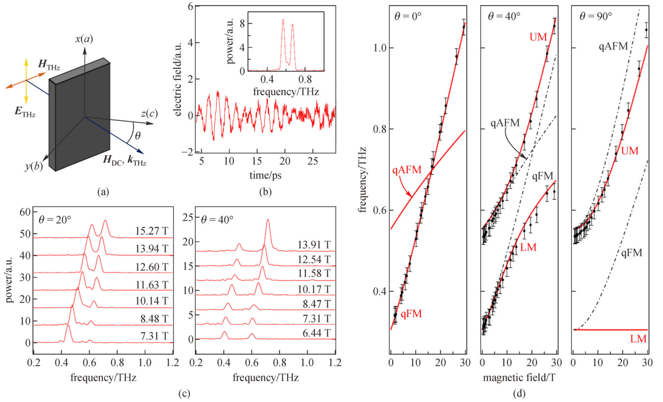
Fig. 9 THz-TDS of magnon-magnon ultrastrong coupling in YFeO_3 evidencing dominant vacuum Bloch–Siegert shifts [42]. (a) Schematic of THz magnetospectroscopy studies of YFeO_3 in a tilted magnetic field. H_{DC} was applied in the b – c plane at an angle of \theta with respect to the c -axis, with k_{THz} \parallel H_{DC} and H_{THz} polarized in the b – c plane. (b) Transmitted THz waveform for \theta = 20^\circ at \mu_0 |H_{DC}| = 12.60 T displaying beating in the time domain and two peaks in the frequency domain. (c) Magnon power spectra for \theta = 20^\circ and \theta = 40^\circ at different H_{DC} , displaying larger frequency splitting for larger \theta . (d) Experimentally measured magnon frequencies for \theta = 0^\circ, 40^\circ, 90^\circ versus \mu_0 |H_{DC}| (black dots) with calculated resonance magnon frequencies (solid red lines) and decoupled qFM and qAFM magnon frequencies (black dashed-dotted lines). The upper mode frequency becomes lower than the qAFM frequency at \theta = 90^\circ , indicating a dominant vacuum Bloch–Siegert shift compared to the vacuum Rabi splitting-induced shift
