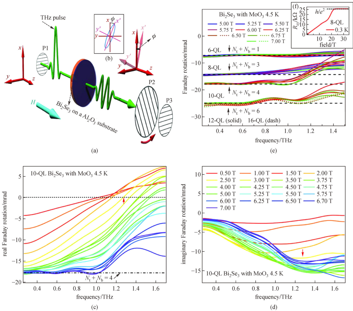
Fig. 6 Quantized Faraday rotation of topological surface states in \text{Bi}_2\text{Se}_3 . (a) Schematic diagram of the Faraday rotation experimental setup. P1, P2, and P3 are polarizers. The polarization acquires an ellipticity simultaneously, as shown in (b). (c) Real part of the Faraday rotation of 10-QL \text{Bi}_2\text{Se}_3 films with \text{MoO}_3 at 4.5 K at various magnetic fields [color-coded as in (d)]. The dash-dotted line is the theoretical expectation. (d) Imaginary part of the Faraday rotation. A representative cyclotron frequency is marked by a red arrow for data at 2.5 T. (e) Quantized Faraday rotation for different samples. Dashed black lines are theoretical expectation values assuming certain values for the filling factor of the surface states. (f) DC Hall resistance of a representative 8-QL sample. Adapted from Ref. [58]
