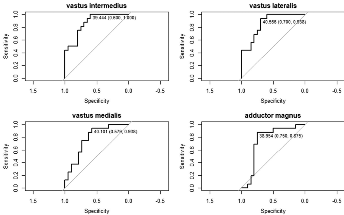
Figure 2 Receiver operating characteristic curve of the sensitivity and specificity achieved by all possible T 2H2O relaxation times. The area under the curve is listed for each plot. In each curve, the threshold with the highest specificity (with zero false positives) and the threshold with optimum sensitivity and specificity are listed.
