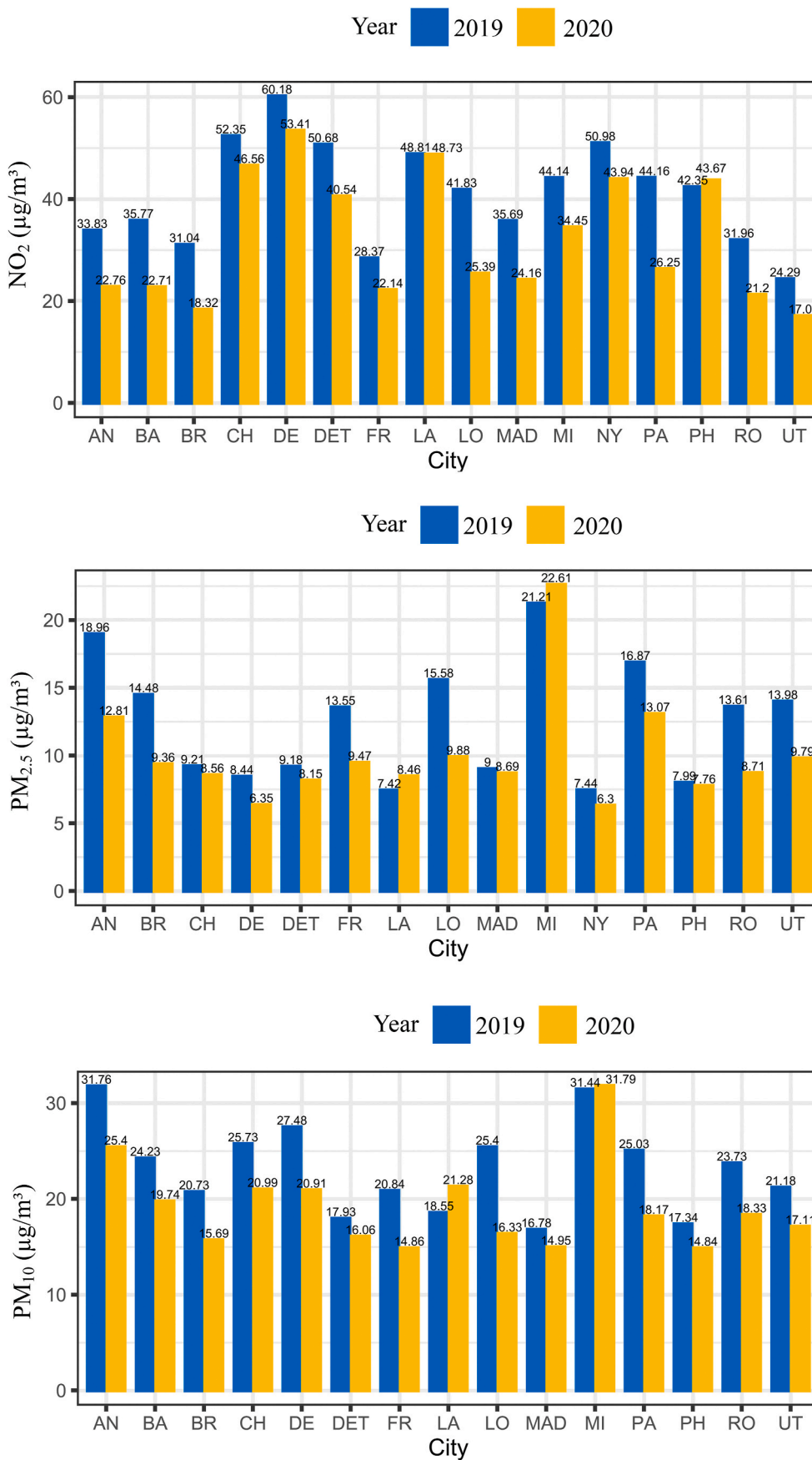
Fig. 6. NO 2 , PM 2.5 , and PM 10 concentration (µg/m 3 ) in selected cities during February 1 to May 11 in 2019 and 2020, derived from in-situ data.
