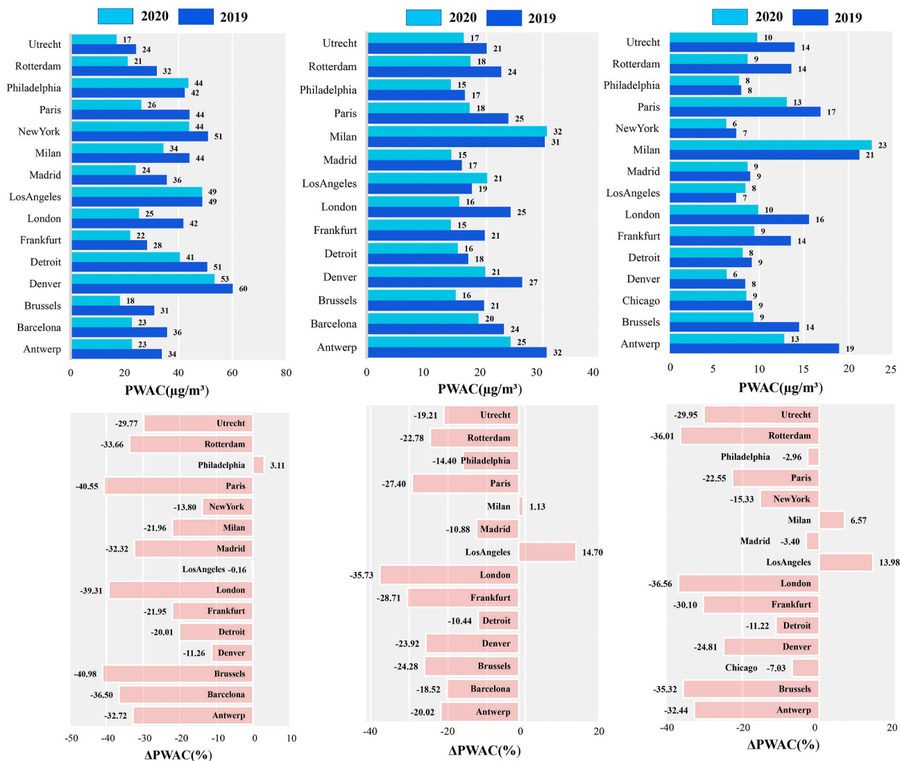
Fig. 9. Population Weighted Average Concentration (PWAC) (µg/m 3 ) for different pollutants in the selected cities.
