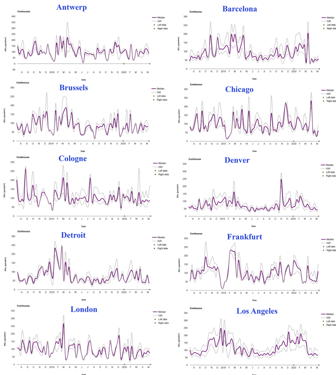
Fig. 4. Temporal variation in NO 2 tropospheric column ( \mu\text{mol}/\text{m}^2 ) in the selected cities, derived from Sentinel 5 P TROPOMI data.
