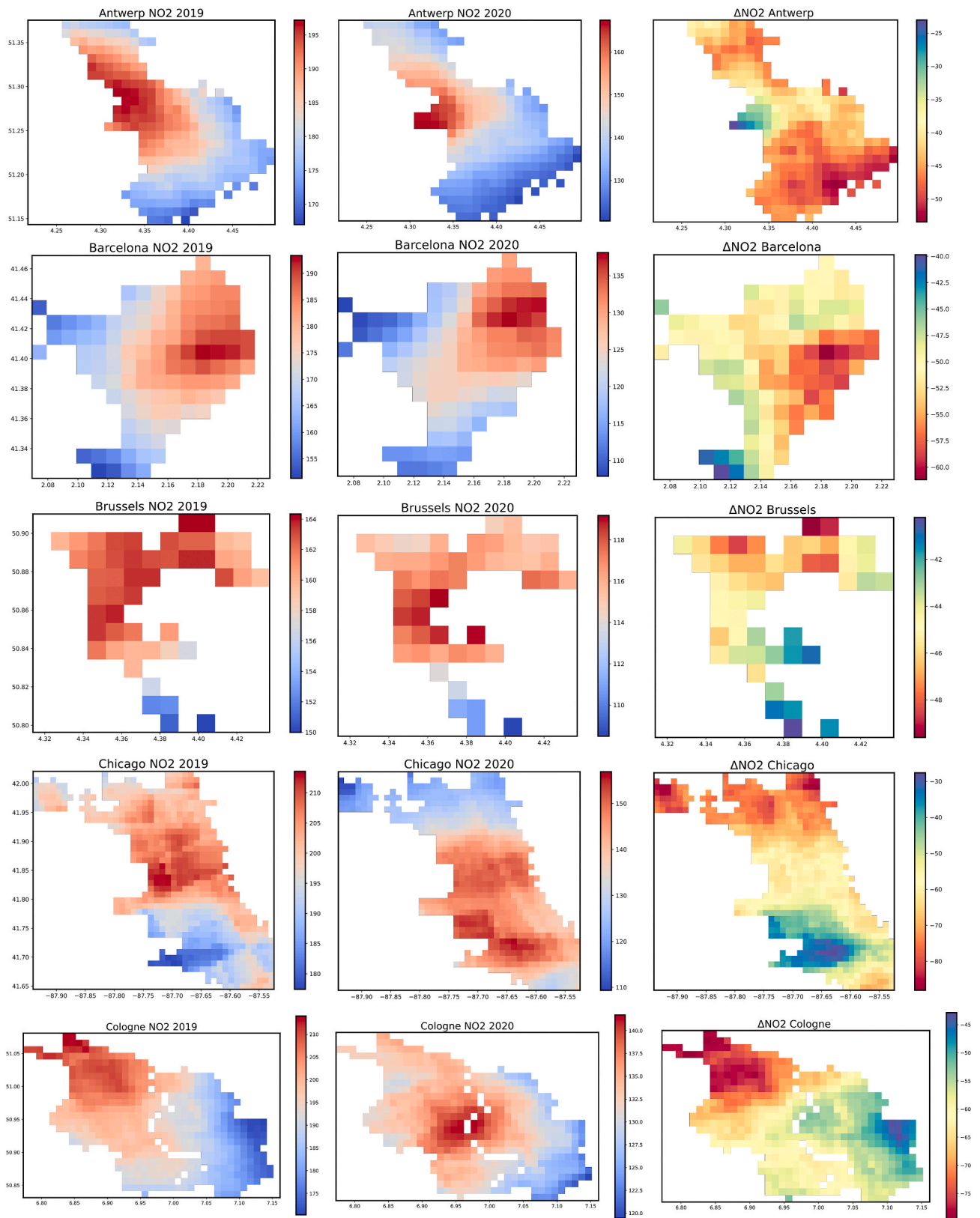
Fig. 1. Spatiotemporal variation (panel a and b) and changes in NO2 tropospheric column ( \mu\text{mol}/\text{m}^2 ) (panel c) in 20 cities during February 1 to May 11 derived from Sentinel 5 P TROPOMI sensor.
