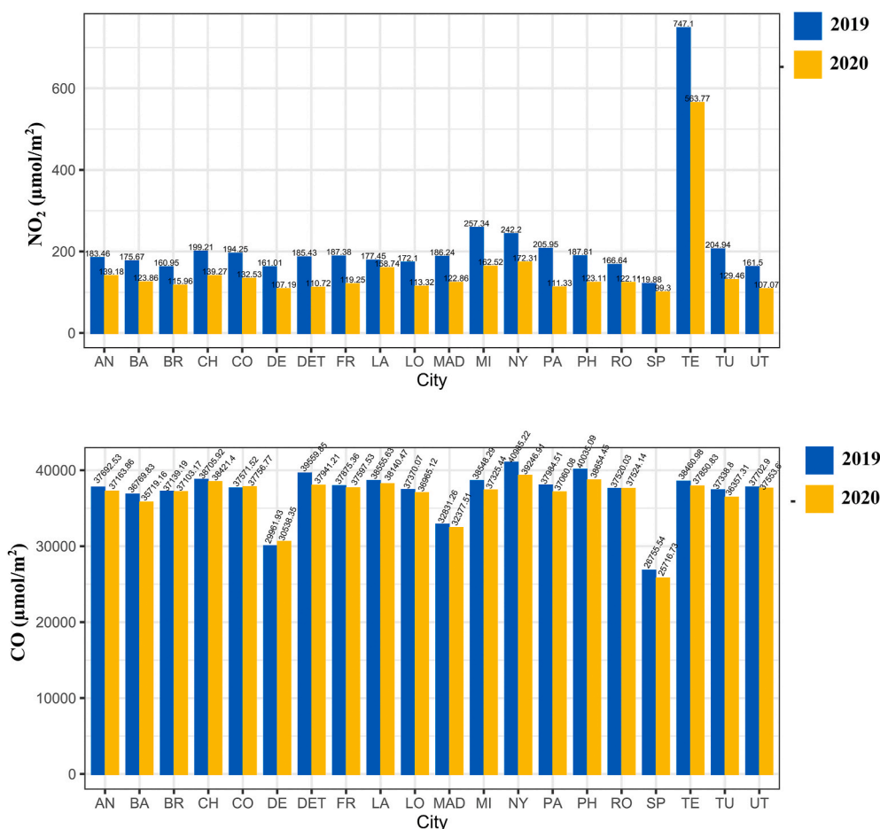
Fig. 2. NO 2 and CO tropospheric column (µmol/m 2 ) in 20 cities during February 1 to May 11 in 2019 and 2020, derived from Sentinel TROPOMI sensor.
