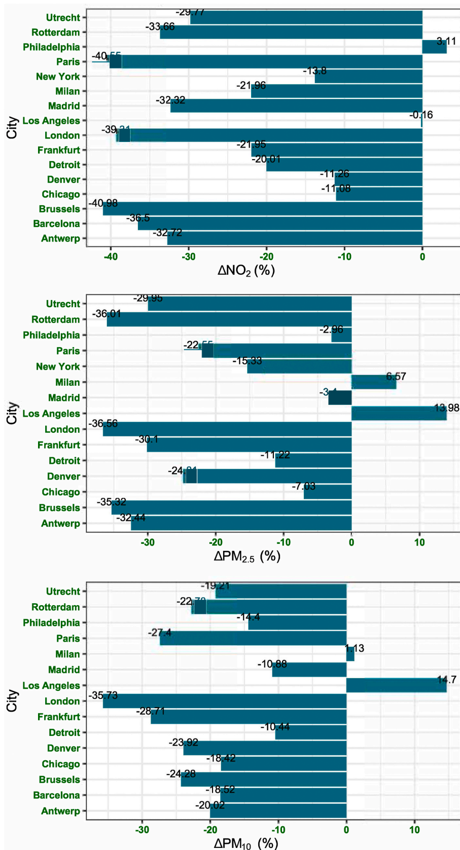
Fig. 7. Changes in NO 2 , PM 2.5 , and PM 10 concentration (%) during February 1 to May 11 in 2019 and 2020, derived from in-situ data.
