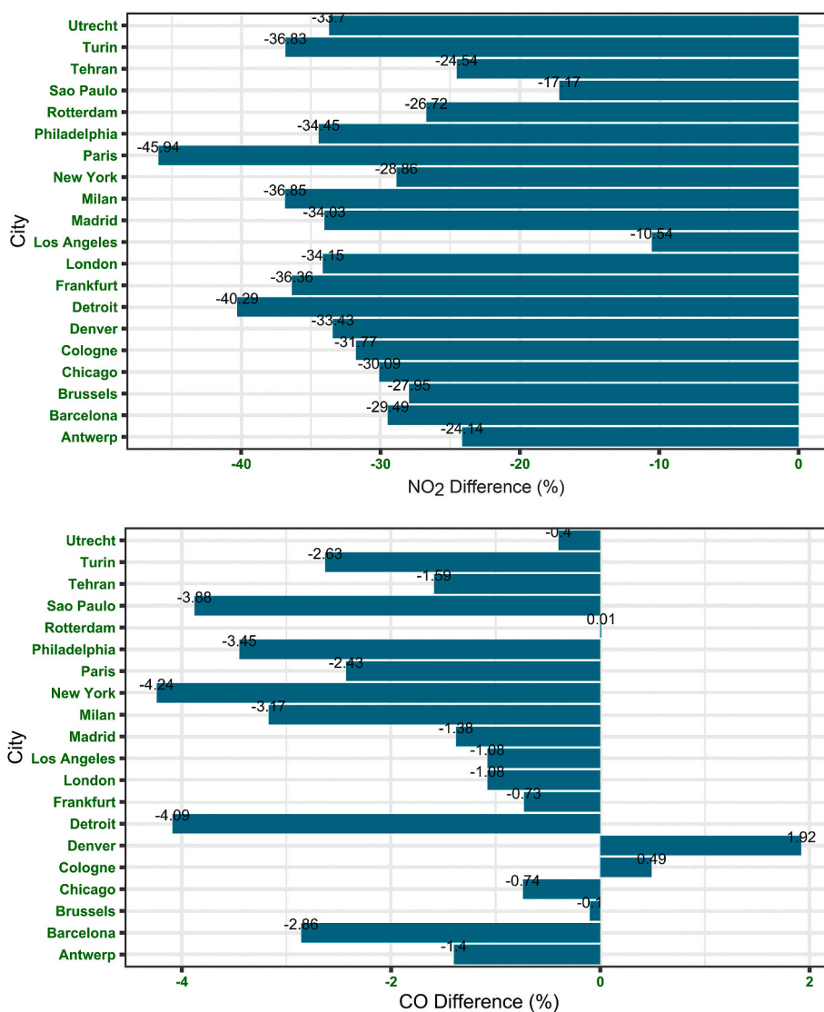
Fig. 3. Changes (%) in NO2 and CO during February 1 to May 11 in 2019 and 2020, derived from Sentinel 5 P TROPOMI data.
