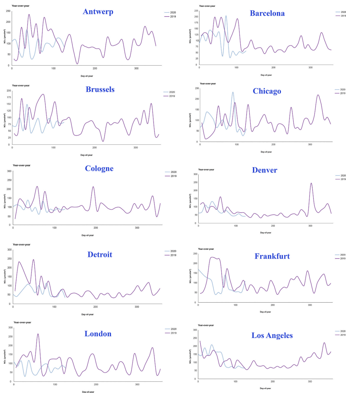
Fig. 5. Variation in NO 2 tropospheric column ( \mu\text{mol}/\text{m}^2 ) in the selected cities during the study period in 2019 and 2020, derived from Sentinel 5 P TROPOMI data.
