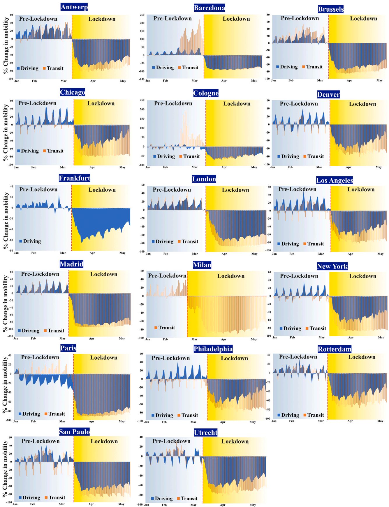
Fig. 8. Changes in mobility due to lock down and resulted in restriction in the selected cities.
