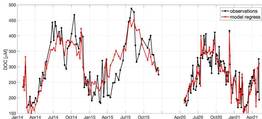
Fig. 4. Time series of DOC observations (black) and values reconstructed by using the stepwise regression model (red).
