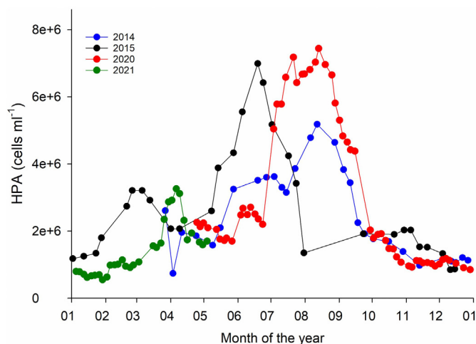
Fig. 7. Annual trend of the heterotrophic prokaryotes abundance (HPA) in 2014, 2015, 2020, and 2021.
