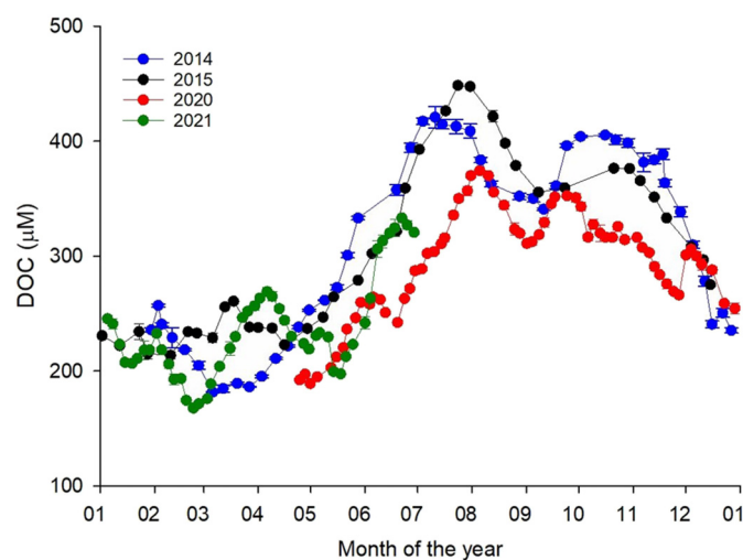
Fig. 3. Arno River DOC concentration in 2014, 2015, 2020, and 2021, bars represent the standard deviation ( n = 3 ).
