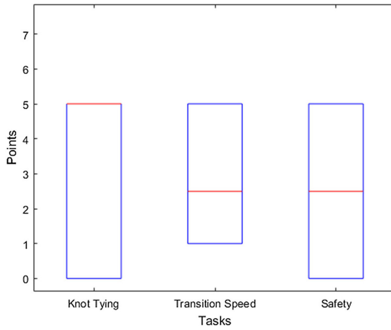
Fig. 4. Distribution of Novice performance results for Knot Tying , Transition Speed and Safety metrics. The highest possible score is 5
