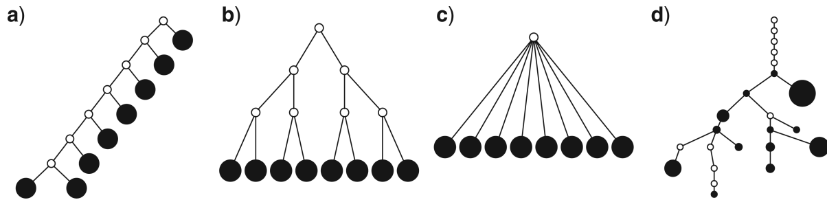
FIGURE 1. Contrasting trees. a) Caterpillar tree with I_S = 35 , I_{S,norm} = 1 , I_C = 21 , I_{C,norm} = 1 , I_\Phi = 56 , I_{\Phi,norm} = 1 . b) Fully symmetric bifurcating tree with I_S = 24 , I_{S,norm} \approx 0.59 , I_C = I_{C,norm} = 0 , I_\Phi = 16 , I_{\Phi,norm} \approx 0.29 . c) Star tree with I_S = 8 , I_{S,norm} = 0 , I_C and I_{C,norm} undefined, I_\Phi = I_{\Phi,norm} = 0 . d) Clone tree of the lung tumor CRUK0065 in the TRACERx cohort (Jamal-Hanjani et al. 2017). In the clone tree, nodes represented by empty circles correspond to extinct clones, and the diameters of other nodes are proportional to the corresponding clone population sizes.
