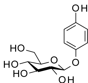
Figure 1. Arbutin (1).
