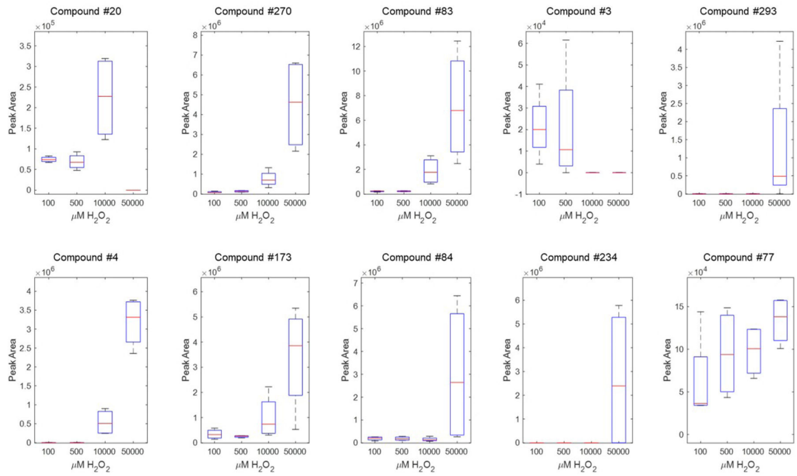
Figure 4. Ten compounds associated with H 2 O 2 exposure per a PLS regression at 12 h H 2 O 2 exposure. Compounds are identified in Table 01
