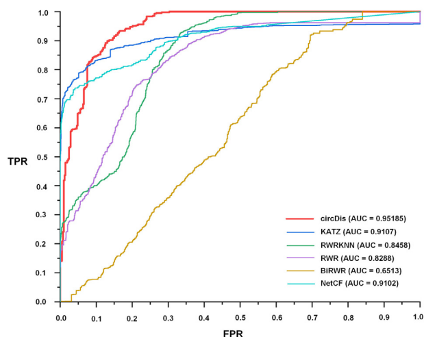
Figure 6 ROC curves and AUC values of the circDis method
