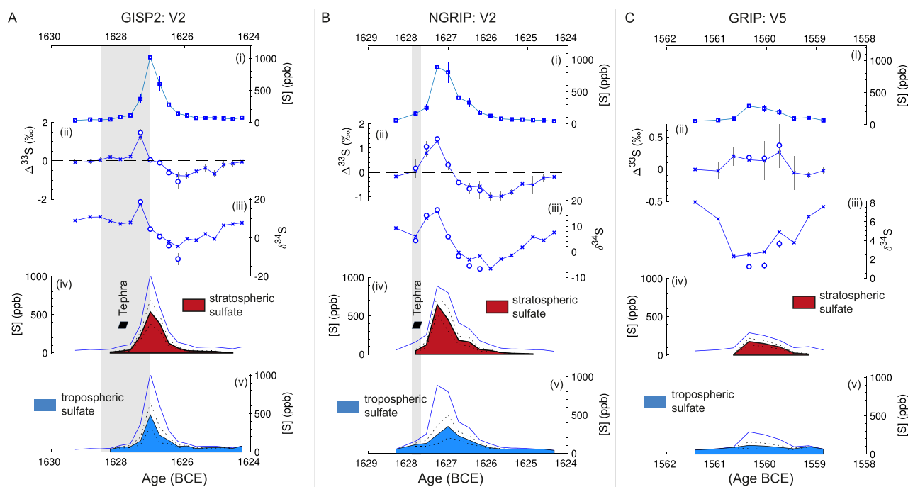
Fig. 5. Sulfur concentration, isotopes, and proportion of stratospheric and tropospheric sulfur from V2 in the GISP2 (A) and NGRIP (B) and V5 in GRIP (C). Each panel illustrates: (i) sulfur concentration (ppb), (ii) measured \Delta^{33}\text{S} in all samples (x's) as well as \Delta^{33}\text{S} of volcanic sulfate (o's), corrected for background sulfate with isotope mass balance for samples with greater than 65% sulfate derived from volcanic sources (see Methods), (iii) same as (ii) but for \delta^{34}\text{S} , (iv) sulfate concentration with the calculated proportion of sulfate deposited via the stratosphere (red), and (v) same as (iv) but blue denotes sulfate that remained below the ozone (mix of background and volcanic sulfate from low atmospheric altitudes). Dotted lines show uncertainties. Tephra shards were found between NGRIP 641.16 and 641.08 m in this study (1627.9 to 1627.9 BCE, see gray vertical bands) partially overlapping in depth with QUB-1198. QUB-1201 (not replicated here), was found between 641.50 and 641.70 m (1631.7 to 1630.5 equivalent).
