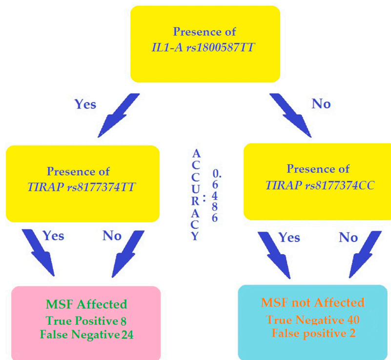
Figure 1. Decision tree algorithm. Data from 292 random selected case (128) and control (164) SNPs typing were used as a training set allow elaborating a decision rule that associates the positivity for one or more SNP genotypes to the MSF-affected and negativity to MSF non-affected label. The better combined decision and leaf nodes generate a decision tree that assign the label using positivity or negativity for the IL-1A rs1800587TT genotype, in the presence or not of TIRAP rs8177374 homozygous genotypes with an accuracy of 0.6486 (accuracy range for the procedure from 0 to 1). Applying the decision tree to the 74 test subjects used as “blinded tests”, only eight of the 32 MSF cases were correctly recognized as MSF patients. On the other hand, 40 out 42 controls used as tests were recognized as healthy.
