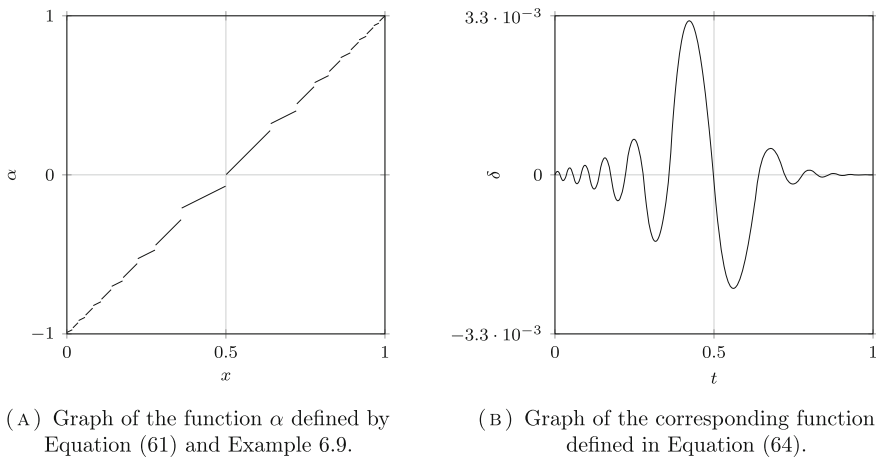
Fig. 10 Plots of the functions of interest in Sect. 6.5
