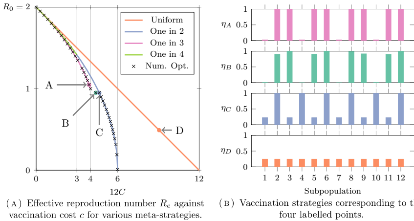
Fig. 3 Pareto frontier and computation of the outcomes for the paths of the four meta-strategies. Some meta-strategies \{\eta_A, \eta_B, \eta_C, \eta_D\} are represented on the right with their corresponding outcome points A–D on the left
