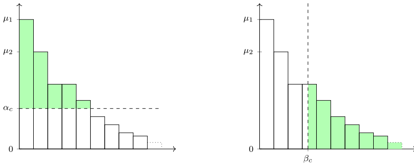
(A) Representation of the greedy path \mathcal{P}_h . (B) Representation of the greedy path \mathcal{P}_v .
