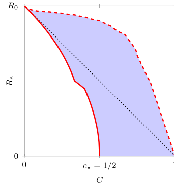
(B) Solid line: the Pareto frontier \mathcal{F} ; dashed line: the anti-Pareto frontier \mathcal{F}^{Anti} ; dotted line: outcomes of the uniform strategies; blue region: all possible outcomes \mathbf{F} .
