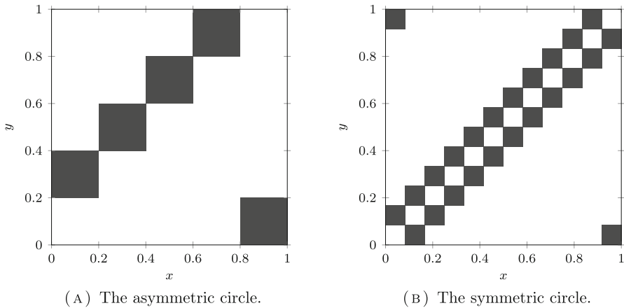
Fig. 4 Kernels k_c (equal to 0 in the white zone and to 1 in the black zone) on \Omega_c = [0, 1] and \mu_c the Lebesgue measure of the continuous model associated to discrete metapopulation models
