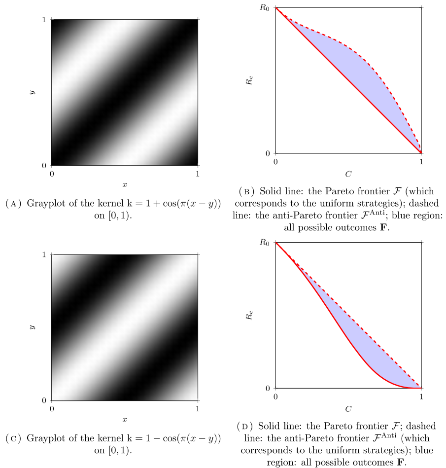
Fig. 12 Two examples of a geometric kernel on the circle \mathbb{R} \setminus \mathbb{Z}
