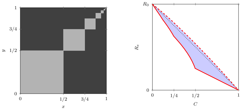
(B) Solid line: the Pareto frontier \mathcal{F} ; dashed line: the anti-Pareto frontier \mathcal{F}^{Anti} ; dotted line: path of the uniform strategies; blue region: all possible outcomes \mathbf{F} .
