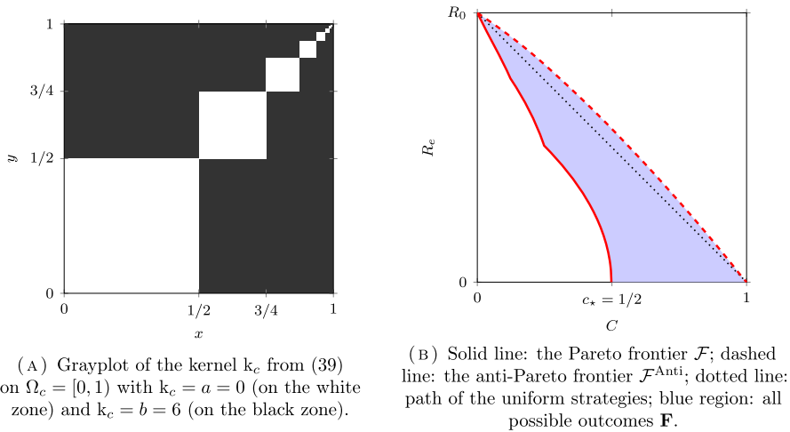
Fig. 8 An example of the complete multipartite model
