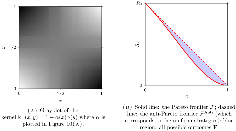
Fig. 11 An example of a constant degree kernel operator of rank two
