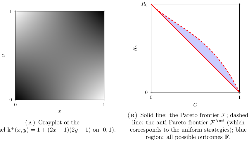
Fig. 9 An example of a constant degree kernel operator of rank two
