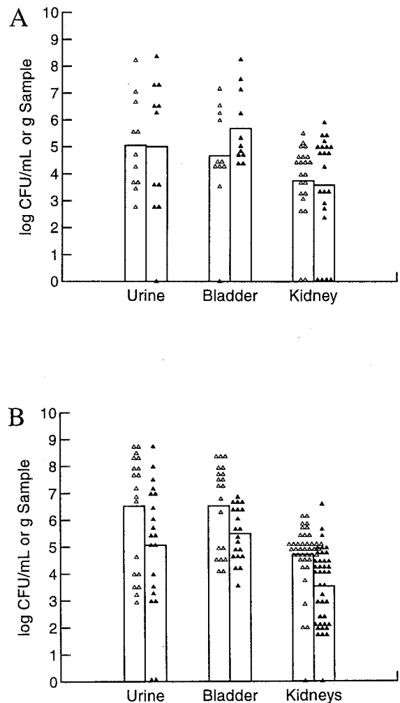
FIG. 5. Mixed infections of C3H/HeOuJ mice. Two strains were mixed in equal numbers and inoculated into female mice. Mice received 2.0 \times 10^8 CFU and were sacrificed 2 days after infection. (A) Mixed infections comparing CP9 (CNF1 + Lac - ) with CP9lacZ (CNF1 - Lac - ). Eleven female C3H/HeOuJ mice were inoculated. Symbols: \Delta , CP9; \blacktriangle , CP9lacZ. (B) Mixed infections comparing CP9lacZ with CP9cnf 1 . Twenty female C3H/HeOuJ mice were inoculated. Counts of CP9lacZ were significantly higher than those of CP9cnf 1 in the urine, bladders, and kidneys (Student's t test, P < 0.05 ). Symbols: \Delta , CP9lacZ, \blacktriangle , CP9cnf 1 . Points represent bacterial numbers in individual samples, and bars represent the means of those samples.
