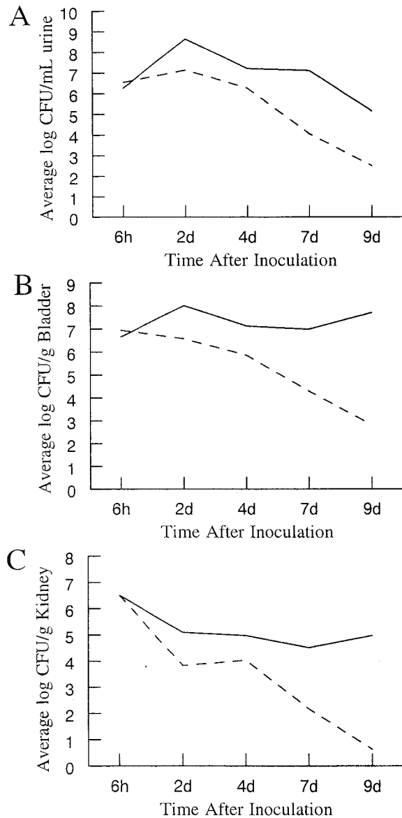
FIG. 6. CNF1 contributes to bacterial survival in a mixed infection. Time courses of mixed infections with CP9 lacZ and CP9 cnf1 are shown. The bacterial strains were mixed in equal numbers, and C3H/HeOuJ mice received 2.0 \times 10^8 CFU. Mice were sacrificed 6 h, 2 days, 4 days, 7 days, and 9 days after infection, and colony counts were performed on collected samples. (A) Mean bacterial numbers in the urine of infected mice. (B) Mean bacterial numbers in the bladders of infected mice. (C) Mean bacterial numbers in the kidneys of infected mice. —, CP9 lacZ ; ---, CP9 cnf1 . Each point represents the mean number of CFU per sample for three mice.
