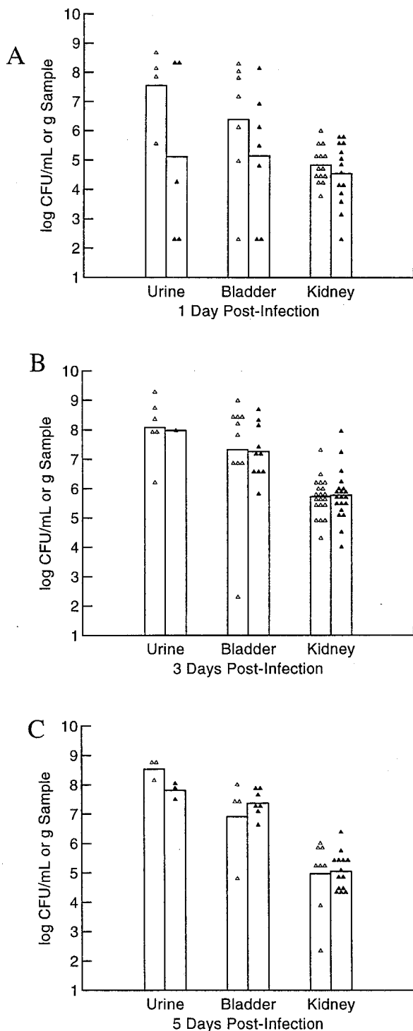
FIG. 2. Kinetics of UTI of C3H/HeOuJ mice with CP9 and the cnf1 isogenic mutant CP9 cnf1 . Thirty female C3H/HeOuJ mice were inoculated transurethrally with 1.9 \times 10^7 CFU of either CP9 or CP9 cnf1 bacteria and sacrificed 1, 3, and 5 days later. Urine, bladder, and kidney samples were recovered, homogenized, and plated for colony counts. Urine samples were not obtained from every mouse, and mice that did not become infected were not included in the analysis. (A) Bacterial counts 1 day after infection. (B) Bacterial counts 3 days after infection. (C) Bacterial counts 5 days after infection. Each point represents one sample. The height of the bar represents the mean for those samples. Symbols: \Delta , CP9; \blacktriangle , CP9 cnf1 .
