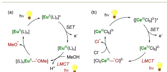
Scheme 7 LMCT-induced homolysis in Eu III /Eu II (a) 146,149 and Ce IV /Ce III (photo)catalysis (b). 90
