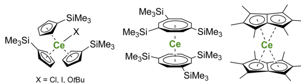
Fig. 5 Examples of Ce IV metallocene complexes.
