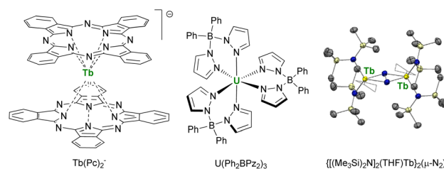
Fig. 6 Molecular structures of Tb(Pc) 2 − , 70 U(Ph 2 BPz 2 ) 3 , 176,177 and ORTEP plot of [(Me 3 Si) 2 N] 2 (THF)Tb) 2 (μ-N 2 ) − , 180 (terbium atoms are in yellow, nitrogen atoms in blue, silicon atoms in pale yellow, carbon atoms in grey, hydrogen atoms are not represented, and coordinated thf molecules are represented in wireframe).
