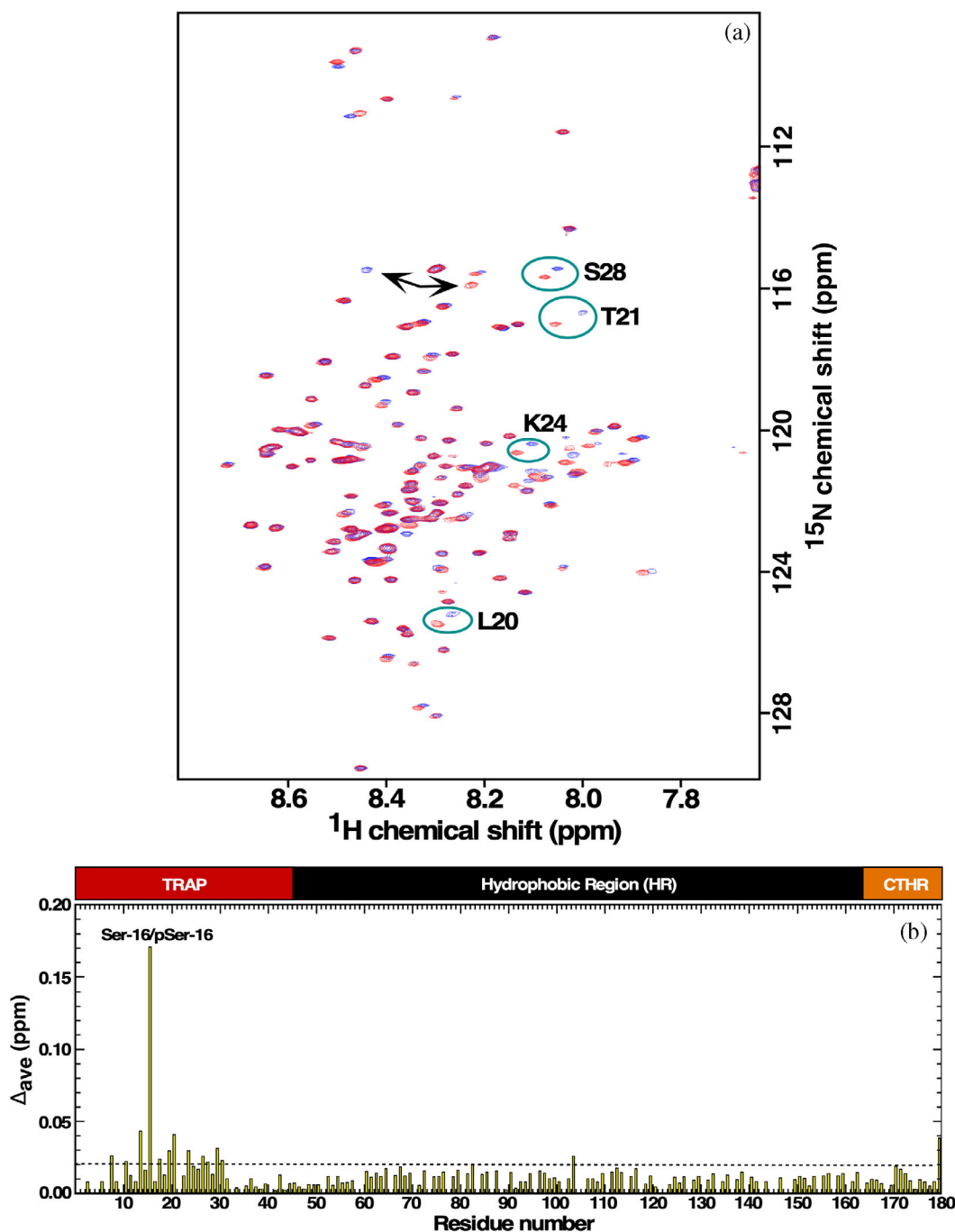
FIGURE 3 (a) Overlay of the ^1\text{H} - ^{15}\text{N} HSQC spectra for ^{13}\text{C} - ^{15}\text{N} -labeled M179 (red) upon pS16M179 (blue) collected in 2% acetic acid (pH 2.8) at 293 K. Spectra were collected on 0.3 mM samples, at a ^1\text{H} resonance frequency of 600 MHz. (b) Plot of the average chemical shift change, \Delta_{\text{ave}} \text{ ppm} = \{[(\Delta^1\text{H}^{\text{N}})^2 + (\Delta^{15}\text{N}/5)^2]/2\}^{1/2} , between the amide resonances of pS16M179 and M179 extracted from ^1\text{H} - ^{15}\text{N} HSQC spectra. The most perturbed resonance is the chemical shift difference between Ser-16 and pSer-16 (labeled with arrows) with mild perturbations confined to a region surrounding pSer-16 in the N-terminal. On top of the plot is a cartoon representation of the three regions present in amelogenin: N-terminal tyrosine-rich region (TRAP; red), hydrophobic region (HR; black) and C-terminal hydrophilic region (CTHR; orange)
