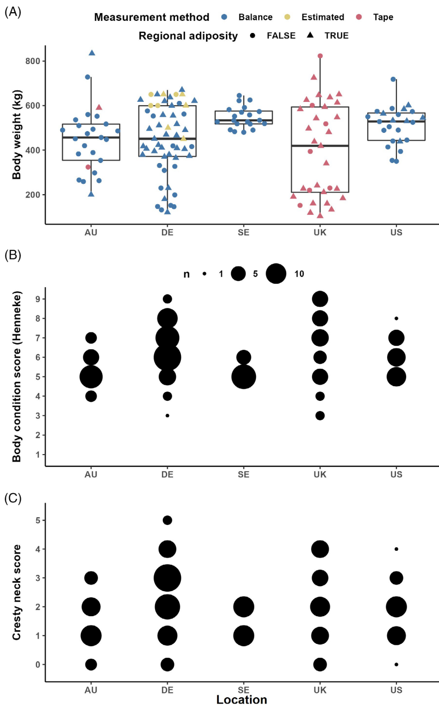
FIGURE 2 Bodyweight (kg) was measured using an electronic balance or weight tape (or estimated in 9 cases) in horses and ponies ( n = 157 ) with a wide range of phenotypes receiving an oral glycemic challenge (A). While the differences in bodyweight between study location were essentially attributable to the breeds included in each cohort, the ponies and horses had body condition scores (B) mostly above 5/9, with more evenly distributed cresty neck scores (C)
