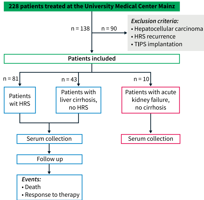
FIGURE 1 Flow chart study design and exclusion criteria.
