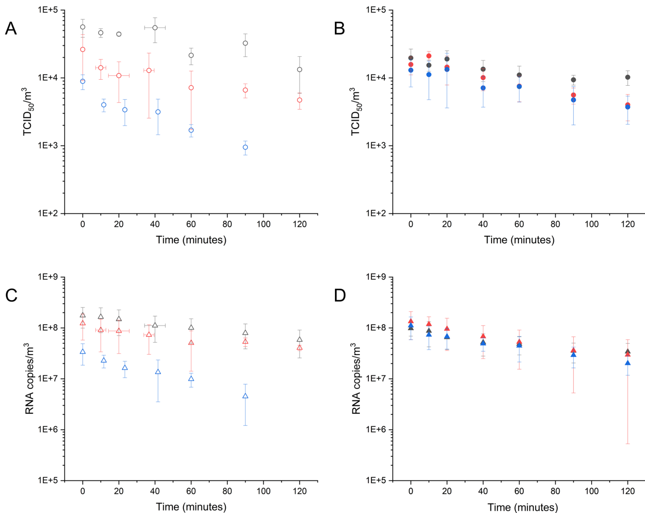
Fig. 3. Time-series (minutes) showing averaged airborne MHV recovery as judged by TCID 50 /m 3 [A and B panels (circles)] and RNA copies/m 3 [C and D panels (triangles)] in the environmental chamber maintained at constant RH for up to 120 minutes. A and C panels (open icons) present airborne MHV recovery aerosolized in DMEM; B and D panels (filled icons) present MHV recovery aerosolized in artificial saliva. Gray icons represent 60% RH conditions; red icons represent 40% RH; and blue icons represent 25% RH conditions. Error bars represent pooled SDs from independent chamber experiments performed in triplicate.
