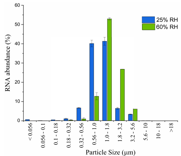
Fig. 2. Particle size distribution of MHV in saliva when aerosolized at 25% RH ( \blacksquare ) and 60% RH ( \blacksquare ) as judged by RNA relative abundance in 11 MOUDI stages. Airborne MHV was aged for 20 minutes at constant RH in the chamber, and RNA was assessed with RT-qPCR.
