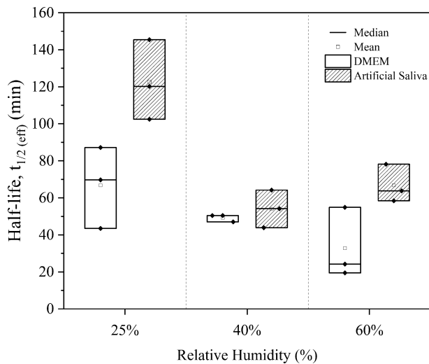
Fig. 1. Effective half-life of airborne mouse hepatitis virus (MHV) based on TCID_{50} recovery from the air contained in a full-scale environmentally controlled chamber (c.a. 10\text{ m}^3 ) at different RH levels; when aerosolized in culture media (DMEM with 2% FBS) ( \square ); and, under otherwise identical conditions in artificial saliva ( \text{▨} ).
