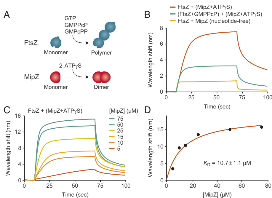
Fig. 1. MipZ binds directly to FtsZ. (A) Schematics depicting FtsZ polymerization in the presence of GTP or its nonhydrolyzable analogs GMPPcP or GMPcPP (Top) and MipZ dimerization in the presence of ATP or its nonhydrolyzable analog ATP \gamma S (Bottom). (B) Biolayer interferometry analysis of the interaction between FtsZ and MipZ. Biotinylated FtsZ immobilized on a streptavidin-coated biosensor was probed with MipZ (15 \mu\text{M} ) in the absence or presence of 1 mM ATP \gamma S or 2 mM GMPPcP. At the end of association phase, the sensor was washed with protein-free buffer to follow MipZ dissociation. Components in parentheses were preincubated together before the start of the binding reaction. Note that 77% of the FtsZ molecules were associated with guanosine-5'-diphosphate (GDP) after purification. (C) Titration series analyzing the interaction of immobilized FtsZ with increasing concentrations (5 to 75 \mu\text{M} ) of MipZ in the presence of ATP \gamma S. (D) Binding affinity of MipZ \cdot ATP \gamma S dimers for FtsZ monomers. The wavelength shifts measured at the end of the association phase ( B_{\text{max}} ) from panel c were plotted against the protein concentration. The apparent equilibrium dissociation constant ( K_D ) of the FtsZ:MipZ complex was obtained by fitting the data to a one-site saturation ligand binding model. The K_D value represents the average of three independent experiments ( \pm SD). The graph shows the results of a representative experiment.
