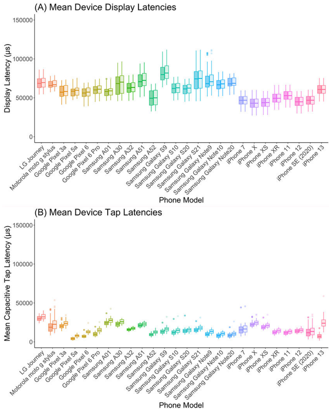
Figure 5. Device Latencies
