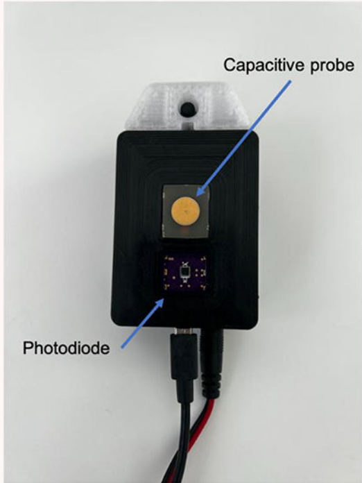
(A) LaTARbot Sensors
