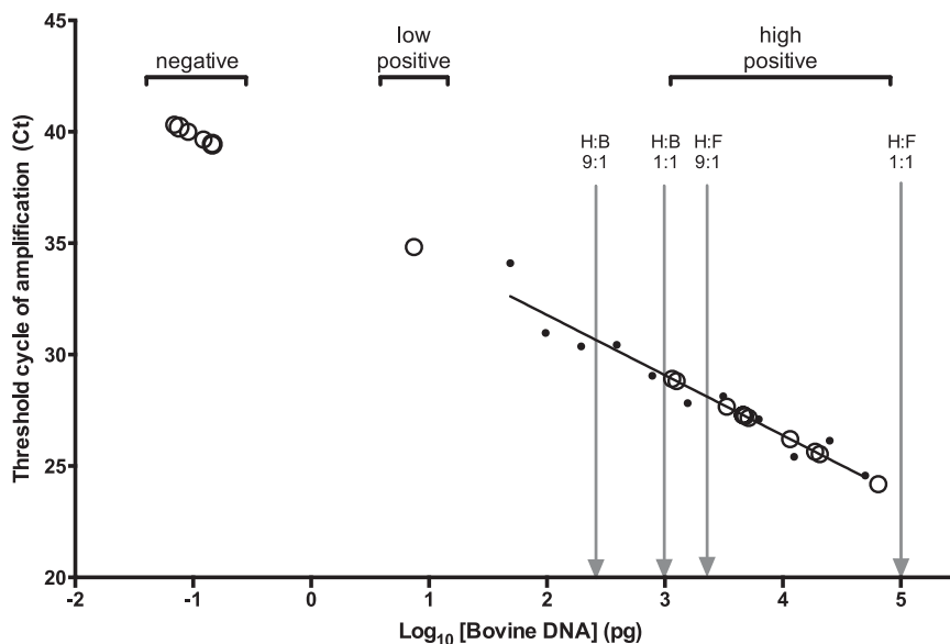
FIGURE 1 Quantification of bovine DNA. The black dots represent a twofold dilution series of total DNA extracted from cow's milk. The solid black line represents the best-fit line and indicates a linear relationship between amplification threshold cycle (Ct) and \log_{10} concentration of bovine DNA. Vertical gray lines indicate the amount of bovine DNA ( \log_{10} ) obtained after mixing reconstituted formula (F) or bovine milk (B) with human breast milk (H), at the indicated ratios (vol:vol). Ct values from 8 bovine-negative and 11 bovine-positive Internet samples are plotted as open circles.
