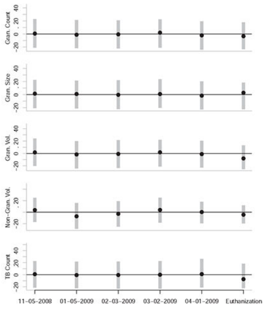
(e) FASL
