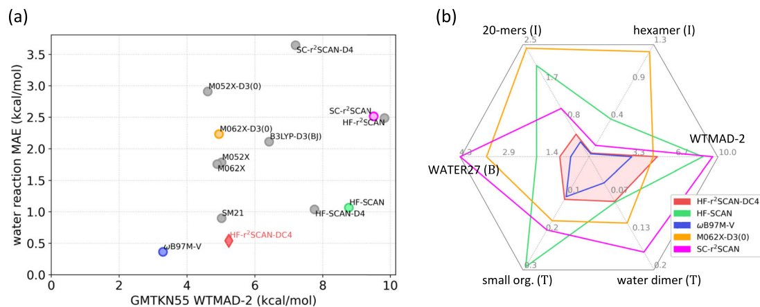
Fig. 5 | Performance of HF-r 2 SCAN-DC4 and other conventional functionals. a The mean absolute error (MAE) for the water-based reactions appear in this work (hexamer isomer energies, water 20-mers isomer energies, WATER27 binding energies, water-small organic molecule interaction energies, and water dimer interaction energies) versus the weighted-mean-absolute-deviation-2 (WTMAD-2) for the GMTKN55 database for selected functionals. For a further description of the reactions used in the y-axis, see Supplementary Note 8. HF-SCAN-D4 functional
