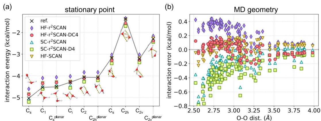
Fig. 2 | Water dimer interaction energies. a Smith stationary points 73 and b MD simulated water dimers with the oxygen-oxygen distance. For a , MAEs of each functional are (following the order in the legend) 0.25, 0.11, 0.09, 0.17, and 0.08 kcal/mol. DLPNO-CCSD(T)-F12 has been used as a reference. For b , MAE of
