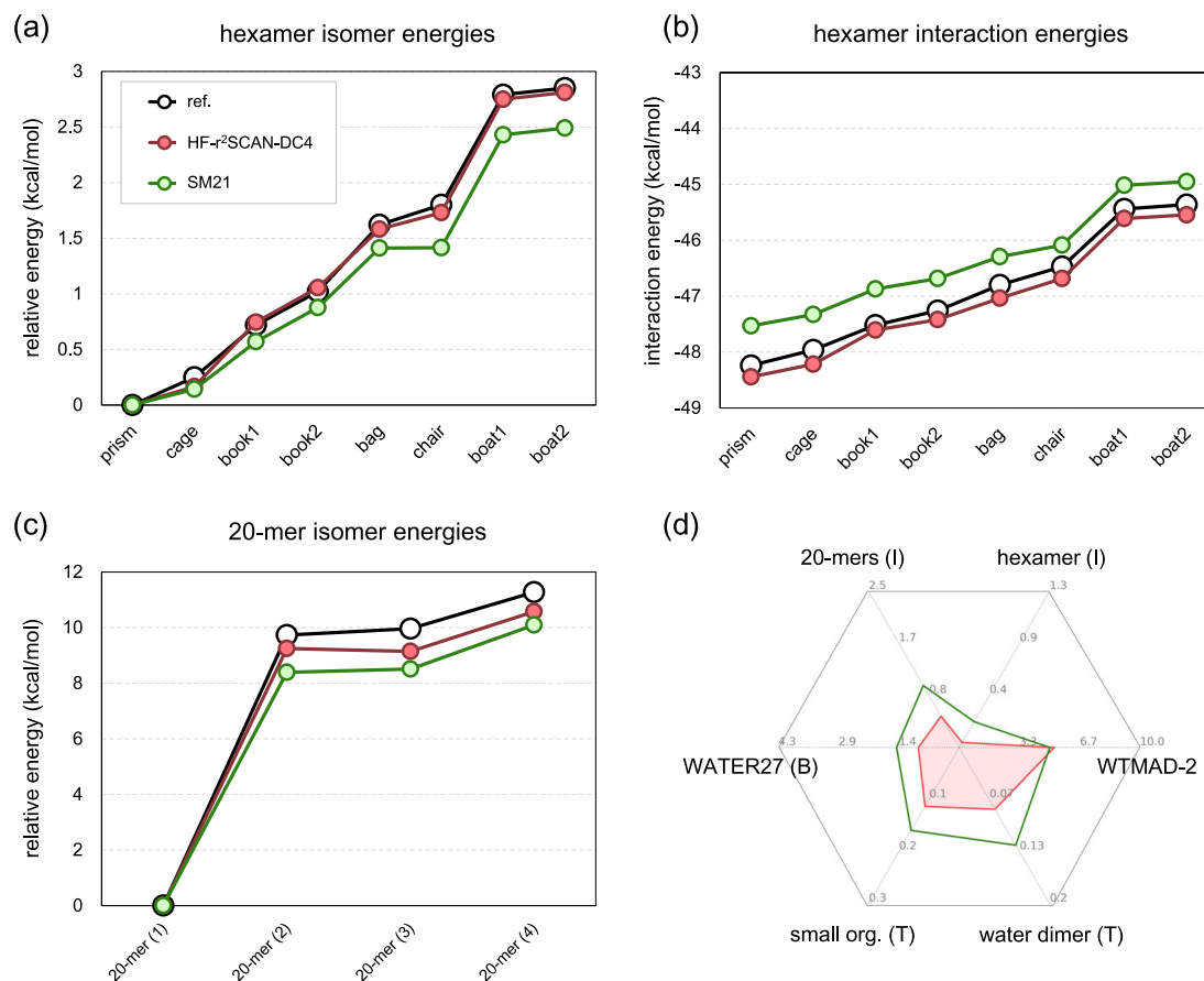
Fig. 6 | Comparison between HF-r 2 SCAN-DC4 and SM21. a Water hexamer isomerization energy, b water hexamer interaction energy, c water 20-mer isomerization energy, and d hexagonal plot same as Fig. 5b. SM21 (green) is HF-r 2 SCAN but with different D4 parameters obtained in ref. 64 .
