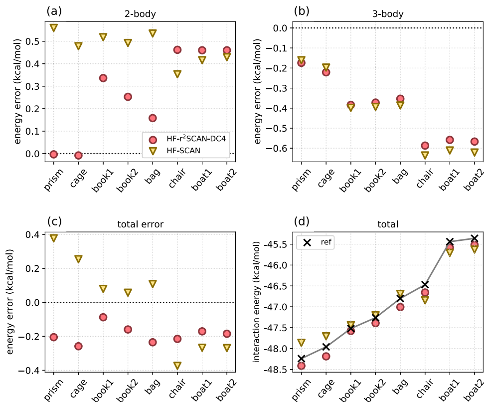
Fig. 3 | K -body interaction energy errors. a K=2 , b K=3 , and c total, and d the interaction energy for 8 water hexamers. (For higher order K -body interaction energies, see Supplementary Figs. 5 and 6.) Geometries and CCSD(T)/CBS reference
