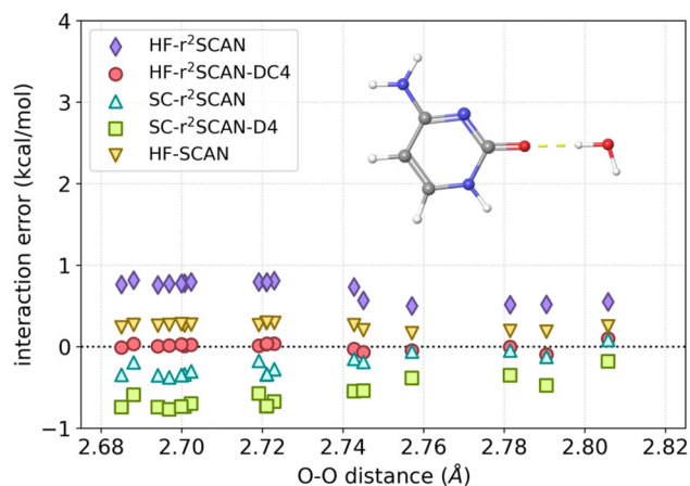
Fig. 4 | Errors in interaction energies of water... cytosine complexes. Atom color code: C, gray; O, red; N, blue; and H, white. Errors are sorted by the distance between the oxygen atom in cytosine and the oxygen atom in water. Reference interaction energies have been computed at the DLPNO-CCSD(T)-F12/AVQZ level of theory.
