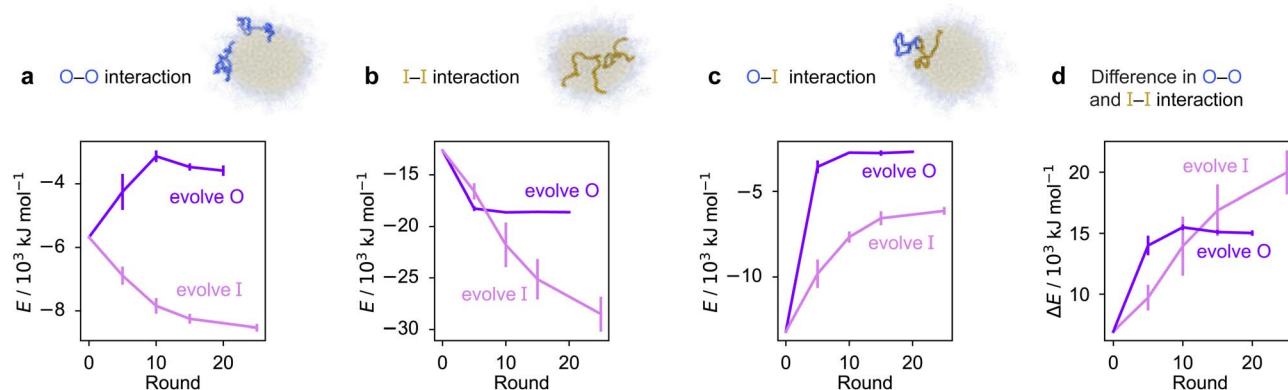
Fig. 4 Homo- and heterotypic interaction strengths control multiphase. The change in the interaction energies of intermolecular homotypic interactions between proteins enriched in the (a) outer and (b) inner layers, (c) heterotypic interactions between the two proteins and (d) the difference between the outer–outer and inner–inner homotypic interactions for the system with the fittest individual. Purple curves correspond to the system where the outer protein was evolved and the inner was unchanged, and pink curves correspond to the converse. Error bars correspond to the standard deviation across three independent runs. Spherical droplets are shown for clarity; we use a slab geometry in direct-coexistence simulations.
