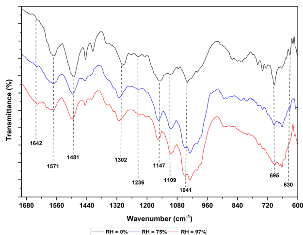
Fig. 2 FTIR spectra of PANi film at RH 0%, RH 75% and RH 97%.
