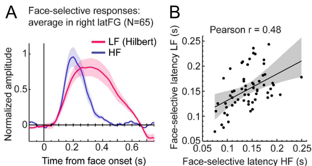
Figure 21. LF and HF timing relationship in the right latFG. (A) Time-domain face-selective responses for LF and HF averaged across 65 recording contacts in the right latFG. The shaded area shows the standard error of the mean across contacts. For LF, to limit the influence of variation in response morphology or polarity across recording contacts, a Hilbert transform was applied to the response of each contact before averaging. Averaged time-domain responses were then normalized (0 to 1) separately for LF and HF and aligned for their pre-face-onset amplitude level (−0.166 to 0 s). (B) Scatter plot showing the relationship between the onset latency of LF and HF face-selective responses measured in individual recording contacts in the right latFG. The shaded area shows the 99% confidence interval of the linear regression line computed by resampling data points with replacement 1000 times.
