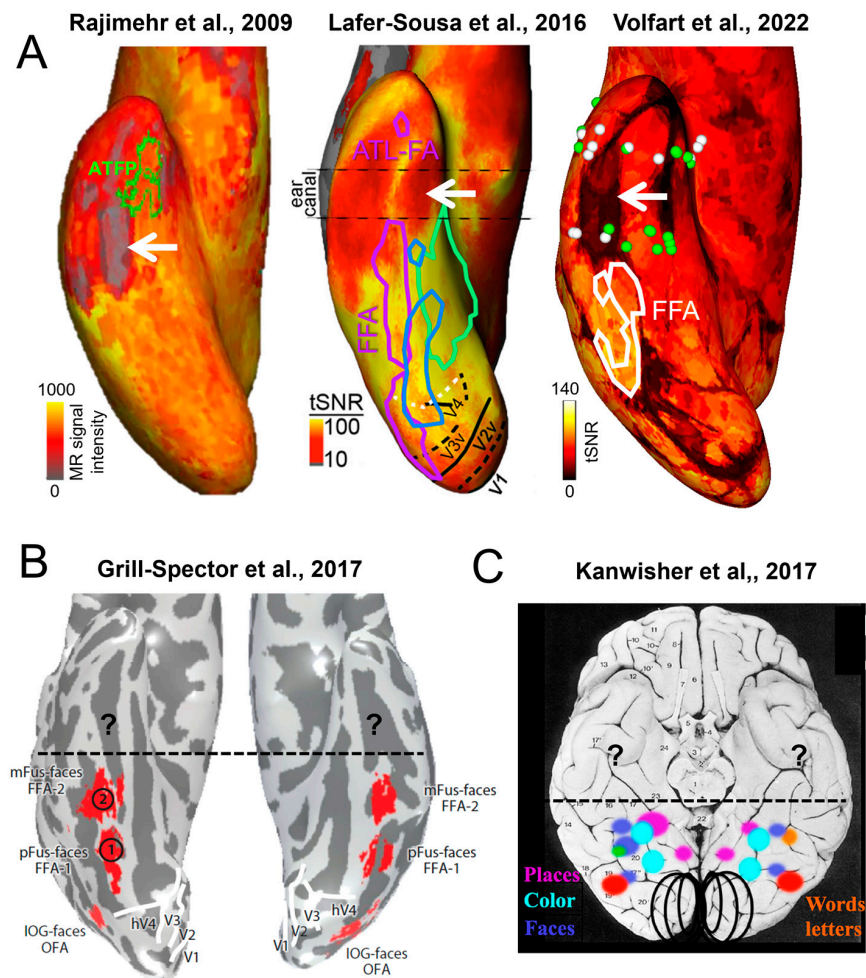
Figure 7. Magnetic susceptibility artifact due to the ear canal (or vATL signal dropout) in fMRI and its consequences on the current picture of fMRI neural basis of human face recognition. (A) These examples show the BOLD signal level and tSNR on ventral views of the inflated cortical surface. The vATL signal dropout is indicated by a white arrow (gray or black zone in Rajimehr et al., 2009 [101]; and in Volfart et al., 2022 [97]; red zone in Lafer-Sousa et al., 2016 [104]; reproduced with permission). In these regions, BOLD measurements are not reliable. Note that face-selective activations (green outlines in Rajimehr et al., 2009, purple in Lafer-Sousa et al., 2016, and white in Volfart et al., 2022) are found all along the VOTC except in the region of the signal dropout. On the contrary, SEEG, which is not affected by SNR variations, is still able to capture face-selective response in this region (green dots in Volfart et al., 2022). (B) Topological organization of the face-selective activations in the VOTC (red spots) in one of the most recent reviews on the functional architecture of face perception in the VOTC (Grill-Spector et al., 2017, [66]). Note that there are no activations anteriorly to the middle fusiform gyrus (FFA, spot indicated by “2” in the figure). (C) Schematic representation (from Kanwisher, 2017 [67]) of the progress made in the understanding of the functional architecture of the VOTC between 1990 (birth of fMRI) and 2017. Although the posterior VOTC is refined (see colored spots representing schematic category-selective regions), little or no progress appears to have been made in mapping anterior VOTC regions with fMRI.
