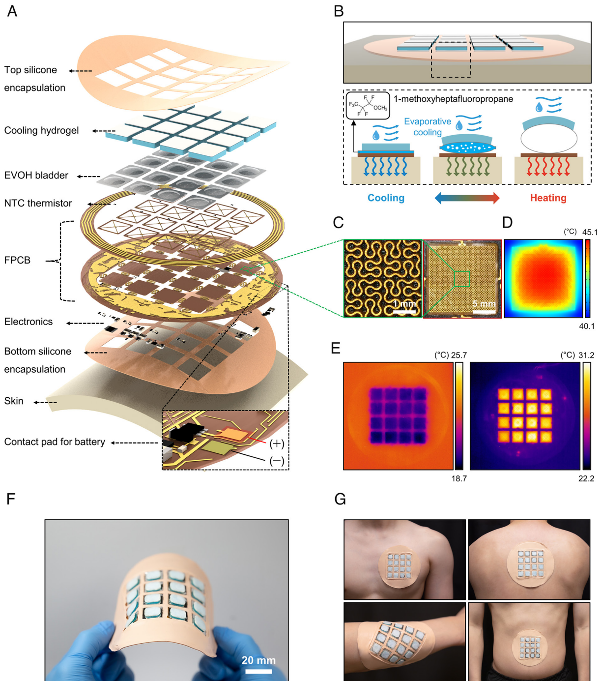
Fig. 1. Design of a thin, flexible, wireless system for generating programmable patterns of thermal sensation across large areas of the skin. (A) Exploded view schematic illustration of a device with 16 independently controlled thermal modules. Each module includes a flexible heater, a negative temperature coefficient (NTC) thermistor, an expandable bladder (as a STB), and a cooling hydrogel. (B) Schematic illustration of the working principle of the device at the skin interface. (C) Photographs of a flexible heater based on Cu traces in a space-filling Peano fractal geometry. (D) FEA simulation result for Joule heating, illustrating a uniform temperature distribution. (E) Infrared (IR) images of a device during the cooling (Left), and heating (Right) mode of operation. (F and G) Photographs of the device (F), and thermal interfaces at various body locations, such as chest, back, forearm, and abdomen (G).
