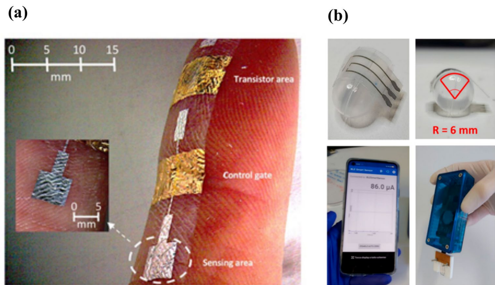
Figure 8. (a): OCMEFET placed on the skin of a finger, demonstrating its good conformability [113]. (b): OECT patterned on polyethylene naphthalate foil bent with a radius of 6 mm to mimic a real-life application; interfacing the sensor with a portable, handheld, battery-powered electronic readout from Elements srl company, wirelessly transmitting the current signal to a smartphone application [115].
