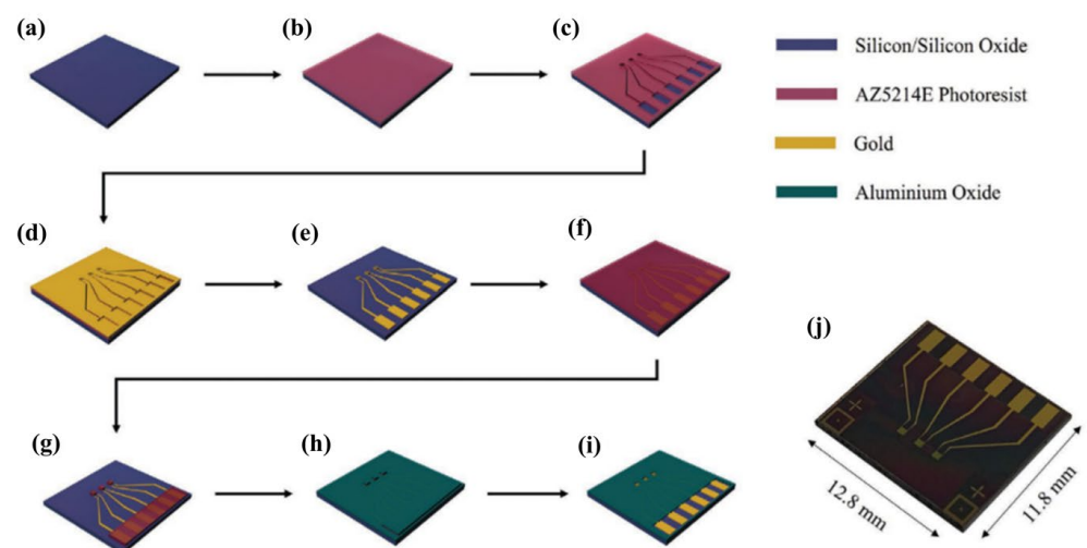
Figure 4. Schematic example of a standard micro-fabrication process employed for EGOT fabrication. (a–e): lift-off process for the definition of source and drain electrodes; (f–i): lift-off process for the definition of contacts passivation. (j) Optical picture of the final device. Copyright (2022) Wiley. Used with permission from M. Segantini et al., “Investigation and Modeling of the Electrical Bias Stress in Electrolyte-Gated Organic Transistors,” Adv. Electron. Mater. , vol. 8, no. 7, 2022, Wiley [59].
