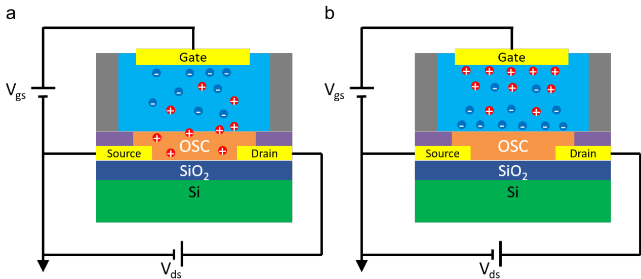
Figure 3. (a): Schematic architecture of an OEET. Application of a positive gate voltage induces cation penetration in the OSC with consequent electrochemical doping. (b): Schematic architecture of an EGOFET. Application of negative gate voltage induces the accumulation of anions (cations) in the EDL at the semiconductor/electrolyte interface, which in turn induces an accumulation of holes (electrons) in the semiconductor.
