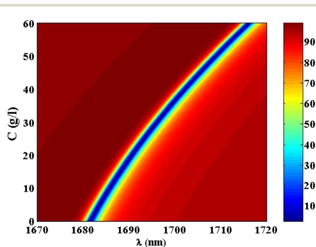
Fig. 7 A color map for the reflectivity of TP resonance at different concentrations of NaCl solution.
