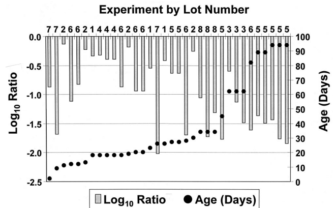
FIG. 3. Comparison of the log of the ratio of stock oocyst count/milliliter and MPN/milliliter with age for all experiments.
