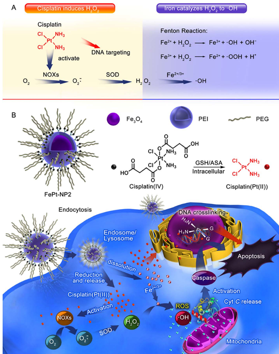
Fig. 3 (A) Cisplatin could activate NOX and catalyze O 2 to form superoxide and H 2 O 2 ; iron ions converted H 2 O 2 to \cdot OH through the Fenton reaction. (B) Iron oxide nanoparticles containing cisplatin(IV) prodrug (FePt-NP2) could activate NOXs and catalyze O 2 to form H 2 O 2 by releasing cisplatin. H 2 O 2 and iron ions generated excess ROS through the Fenton reaction, resulting from rapid lipid and protein oxidation and DNA damage, and triggering the ROS/CytC/caspase-3 pathway leading to apoptosis. Reproduced with permission. 61 Copyright 2017, American Chemical Society.
