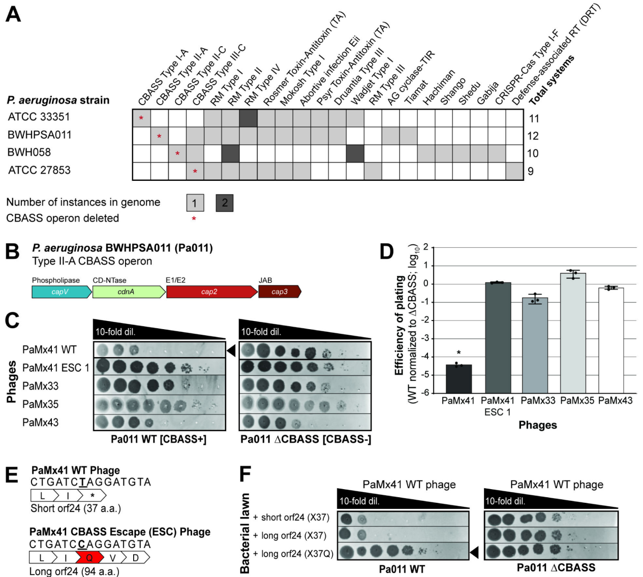
Figure 1. P. aeruginosa BWHPA011 (Pa011) CBASS-based immunity protects against PaMx41 infection. (A) The presence of different anti-phage immune systems in P. aeruginosa strains that were used in this study. Some systems are present in the genome twice as indicated by the darker shade of gray and number (2). An asterisk (*) indicates the CBASS operon was effectively deleted from the bacterial genome. (B) Pa011 CBASS operon. (C) Plaque assays with PaMx41-like phages and an evolved PaMx41 CBASS Escaper (ESC) phage spotted in 10-fold serial dilutions on a lawn of Pa011 WT [CBASS+] or ΔCBASS [CBASS-]; clearings represent phage replication. Black arrowhead highlights the reduction in PaMx41 WT phage titer. See also Figure S1. (D) Efficiency of plating was quantified as plaque-forming units (PFU) per ml on Pa011 WT divided by PFU/ml on the ΔCBASS (n=3). Data are mean ± s.d. Non-parametric ANOVA test yielded a P value of <0.0001. (E) Schematic of PaMx41 WT and CBASS escape phage genomes with the no-stop extension mutation. The bold underline indicates mutation of thymine (T) to cytosine (C), resulting in a stop codon (TAG, *) to
