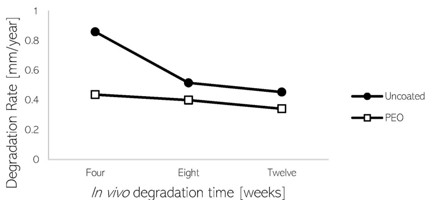
Fig. 4. A) 3D rendering of a 4-week degraded PEO-coated screw surrounded by trabeculae bone created in Avizo. Non-degraded WE43 material is segmented in blue and surrounding non-metallic material in white (bone and degradation layer). B) In vivo degradation rates of uncoated and PEO-coated screws after 4, 8, and 12 weeks calculated from segmented \mu CT data.
