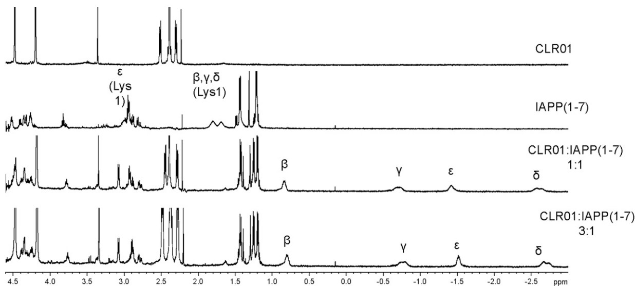
Fig. 6. CLR01 binding induces a massive upfield shift of Lys sidechain protons inside its cavity. ^1\text{H-NMR} spectra were recorded for CLR01, IAPP(1–7), and their 1:1 or 1:3 complexes in 10 mM phosphate-buffered \text{D}_2\text{O} , pH 7.2. The Lys1 side-chain methylene signals are assigned as \alpha , \beta , \gamma , \delta , and \epsilon . All the methylene resonances, most notably the \delta - and \epsilon -protons, are shifted upfield by 4.4 and 4.5 ppm, respectively, indicating strong binding of CLR01 to Lys1.
