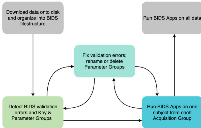
Fig. 1. CuBIDS workflow.
