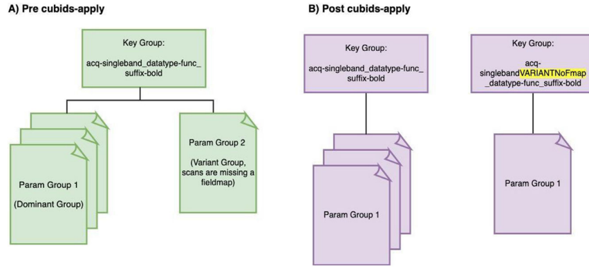
Fig. 3. Parsing the dataset by Parameter Group.
