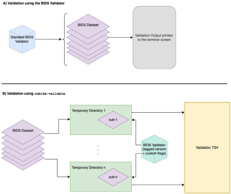
Fig 2. Stable, scalable BIDS validation.
