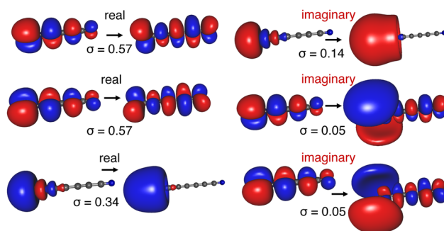
FIG. 17. Real and imaginary NTOs for the {}^1\Sigma^+ resonance in \text{C}_7\text{N}^- . This state has mixed \pi \rightarrow \pi^* and \sigma \rightarrow \sigma^* character, as apparent from the participation ratio \text{PR}_{\text{NTO}}(\gamma^{\text{Re}}) \approx 3 . Based on the singular values \sigma_K^{\text{Im}} , the total width of 0.13 eV can be separated into two contributions, \Gamma_\Sigma = 0.10 eV and \Gamma_\Pi = 0.03 eV, corresponding to the two decay channels in which the \text{C}_7\text{N} radical is either formed in the {}^2\Sigma^+ or the {}^2\Pi state. Reprinted with permission from W. Skomorowski and A. I. Krylov, J. Phys. Chem. Lett. 9 , 4101 (2018). Copyright 2018 American Chemical Society.
