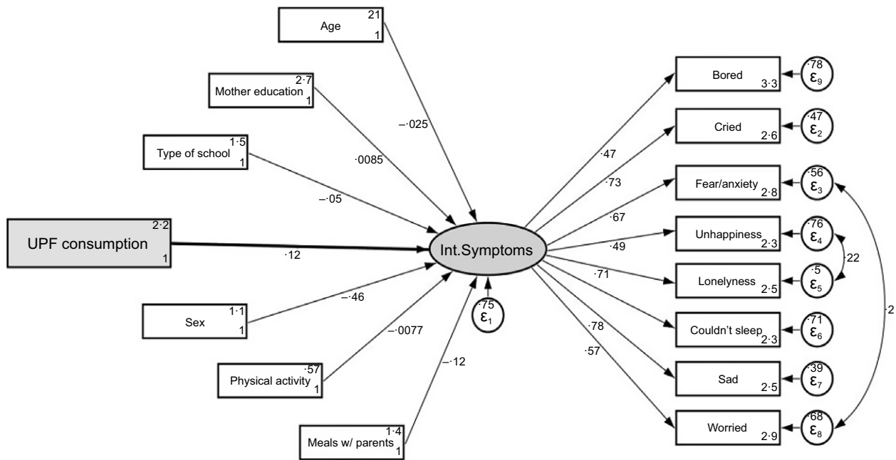
Fig. 2 Structural equation models for the adjusted association between ultra-processed food (UPF) consumption and internalising symptoms behaviors among adolescents in São Paulo (n 2680), Brazil, 2017
