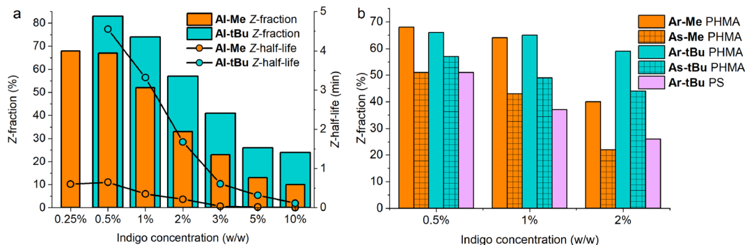
Fig. 4 (a) Z-Fractions upon excitation with 660 nm light and thermal Z half-lives of Al-Me and Al-tBu , and (b) Z-fractions of Ar-Me , As-Me , Ar-tBu and As-tBu at different dye loadings in PHMA and Ar-tBu in PS.
