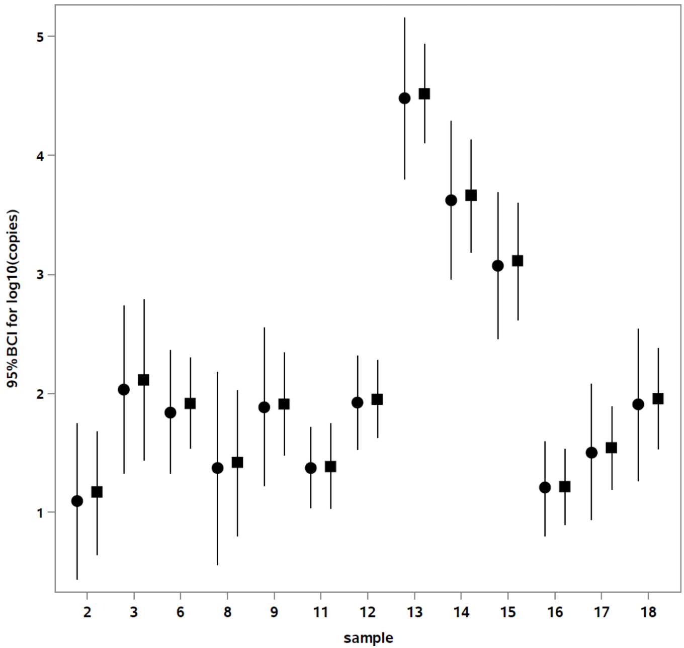
Fig. 3. Overall mean log 10 copies plus 95% BCI per reaction for balanced data from 11 laboratories. ●: Ct calibration model, ■: Master Standard Curve calibration model.
