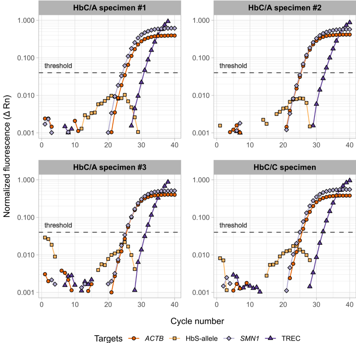
S3 Figure. Amplification plots for four exemplary HbC-containing specimens devoid of HbS (three HbC/A and one HbC/C). The signal for the HbS allele is not amplified in any of the samples. The corresponding MS/MS results are shown in S4 Table.
