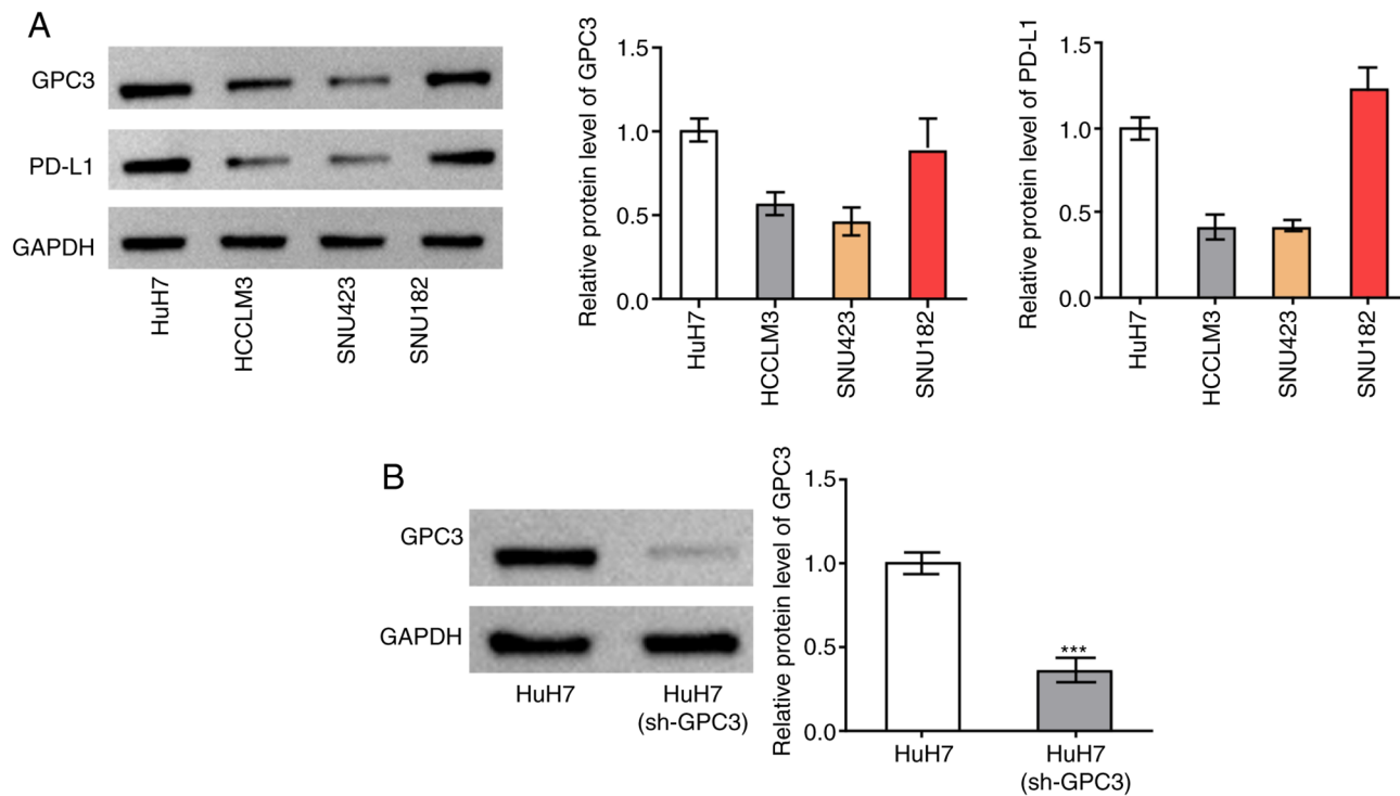
Figure S1. GPC3 and PD-L1 are expressed in HCC cell lines. (A) The expression of GPC3 and PD-L1 in SNU182, HCCLM3, HuH7 and SNU423 cells was detected using western blotting. (B) GPC3 expression was knocked down in HuH7 cells via GPC3 shRNA transfection. Data are presented as the mean \pm SD. *** P <0.001. GPC3, glypican-3; PD-L1, programmed death ligand 1; HCC, hepatocellular carcinoma.
