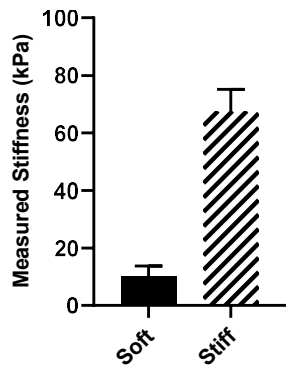
Figure S1. PA gel elastic modulus measurements via contact mode atomic force microscopy. Measurements were performed following the protocol outlined in the STAR methods section. Error bars represent mean \pm SD for measurements taken at 16 locations in each gel within a 120x120µm grid.
