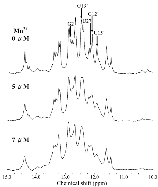
Figure S1. Changes in ^1\text{H} spectra in the imino proton region upon titration of Rz-3 with \text{MnCl}_2 . ^1\text{H} spectra of Rz-3 (0.2 mM) were measured in the presence of 0, 5 and 7 \mu\text{M} \text{MnCl}_2 at 25°C.
